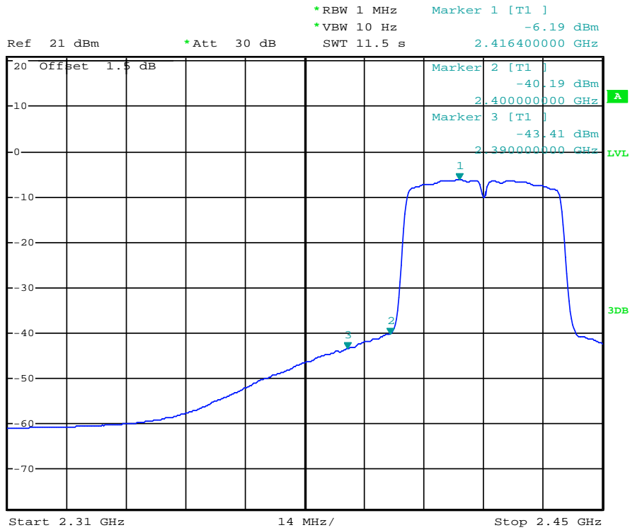
(Plot 4.5.4 A1: Channel 3: 2422MHz @ 802.11n(40MHz))
