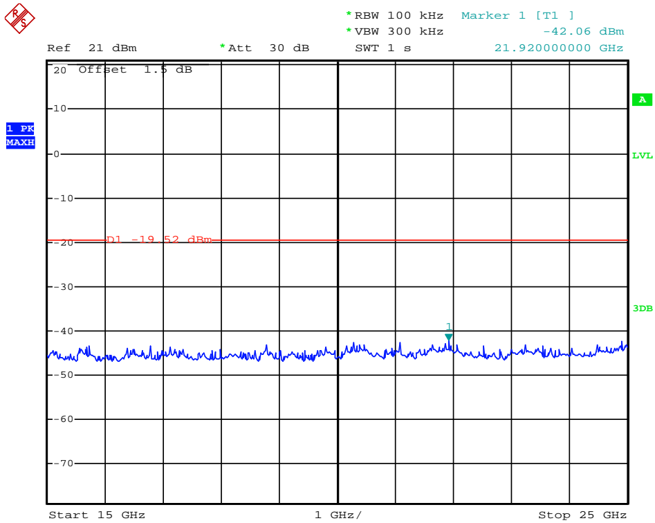
(Plot 4.9.1.C2: Channel 78: 2480MHz @ GFSK)
