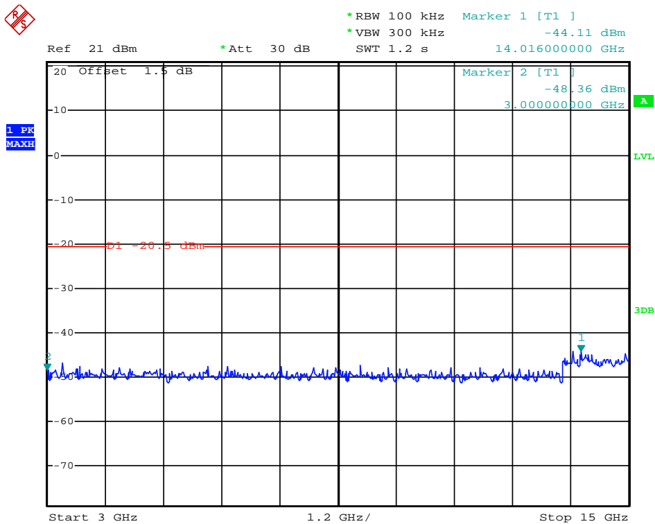
(Plot 4.9.3.B1: Channel 39: 2441MHz @ \pi/4 QPSK)
