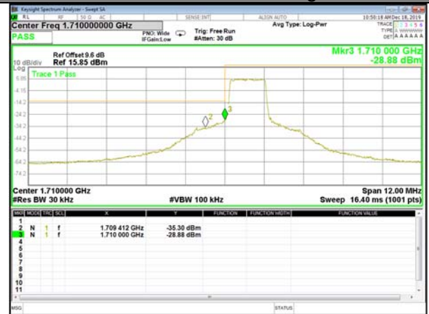
16QAM_1.4M_Lower_Band edge_Full-RB
