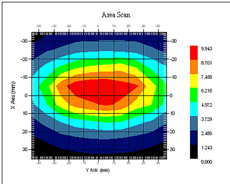
835 MHz System Validation
