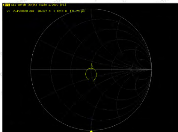
Impedance Test-Body
