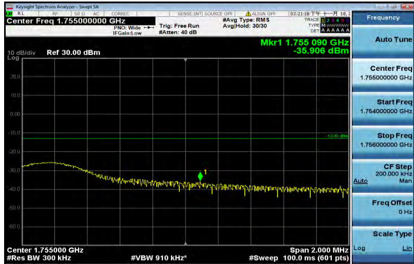
Band4-15MHz-16QAM-20325-1RB#74
