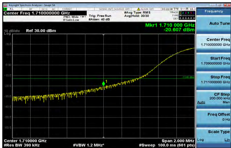
Band4-20MHz-16QAM-20050-100RB#0
