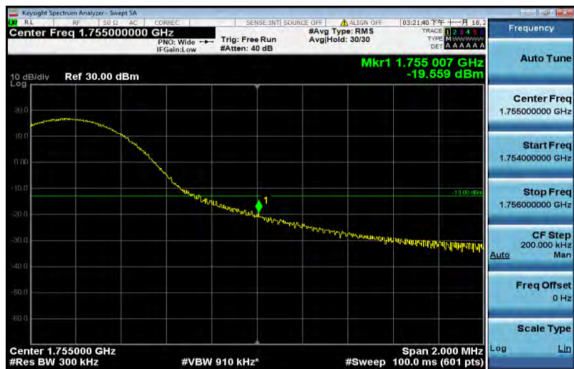
Band4-15MHz-16QAM-20325-75RB#0
