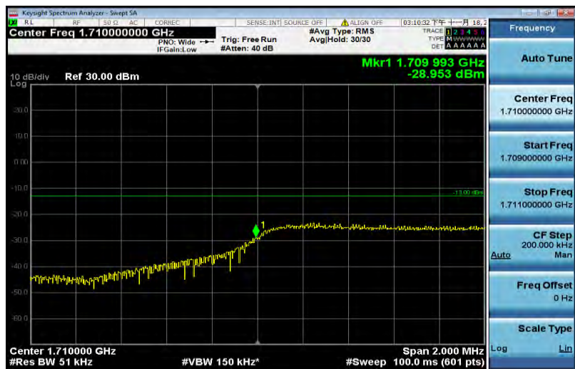
Band4-3MHz-QPSK-19965-15RB#0
