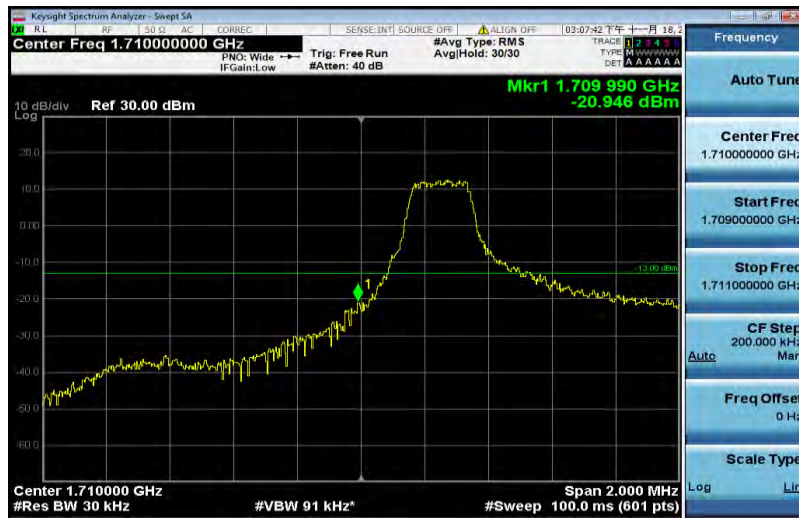
Band4-1.4MHz-QPSK-19957-1RB#5
