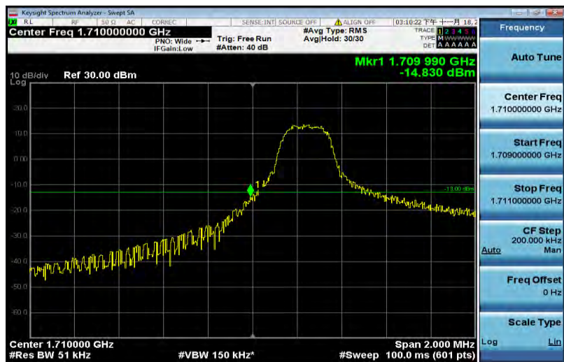
Band4-3MHz-16QAM-19965-15RB#0
