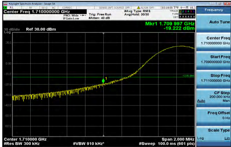
Band4-15MHz-16QAM-20025-1RB#74
