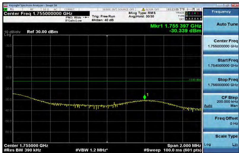
Band4-20MHz-QPSK-20300-100RB#0
