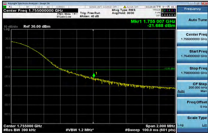
Band4-20MHz-QPSK-20300-1RB#0
