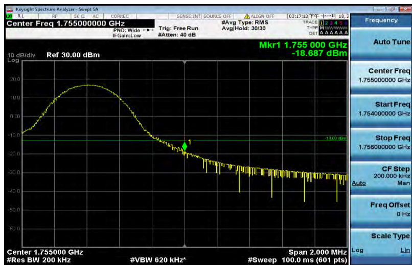
Band4-10MHz-QPSK-20350-50RB#0
