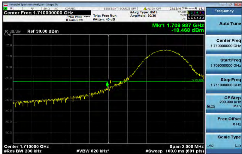
Band4-10MHz-16QAM-20000-1RB#49
