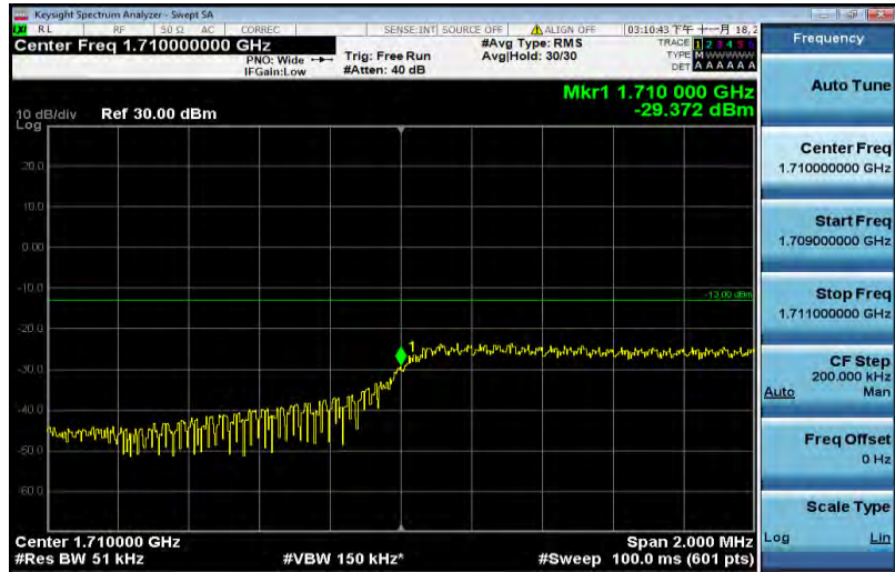
Band4-3MHz-16QAM-19965-1RB#0
