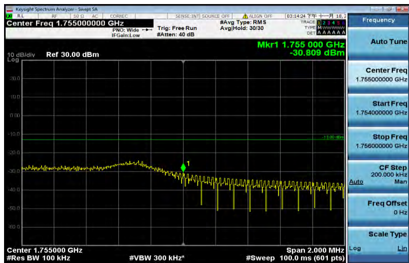
Band4-5MHz-QPSK-20375-25RB#0
