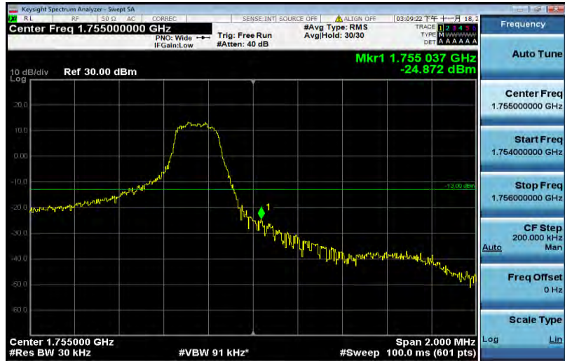
Band4-1.4MHz-QPSK-20393-1RB#0
