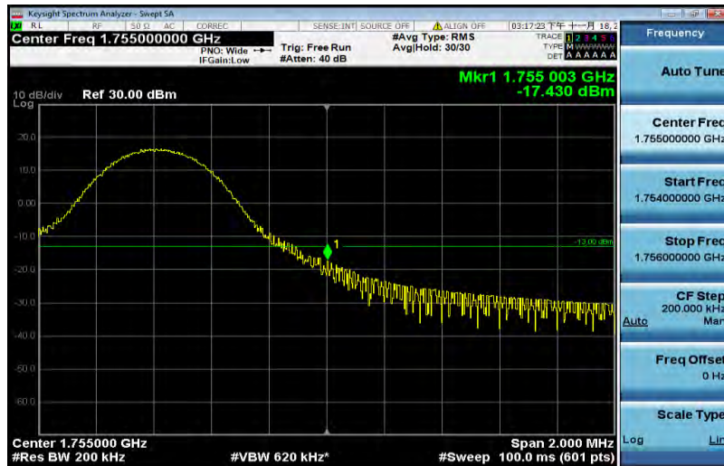
Band4-10MHz-16QAM-20350-1RB#0
