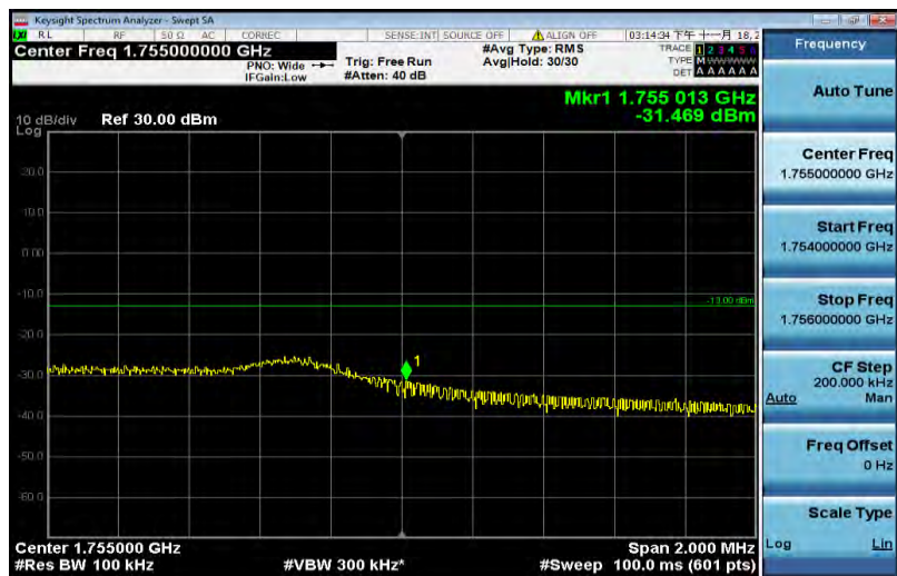
Band4-5MHz-16QAM-20375-25RB#0
