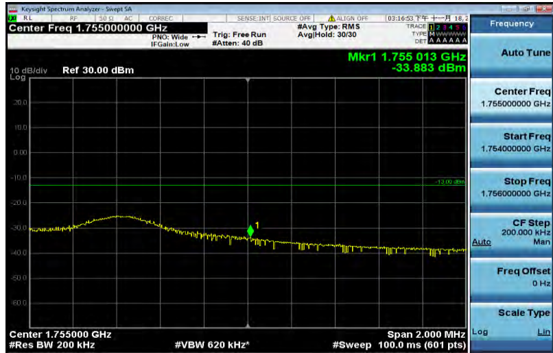
Band4-10MHz-QPSK-20350-1RB#49
