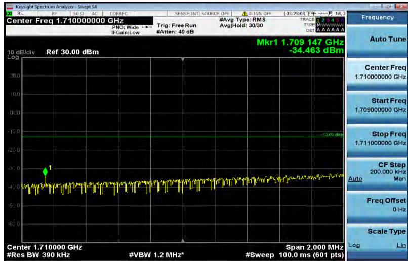
Band4-20MHz-16QAM-20050-1RB#0
