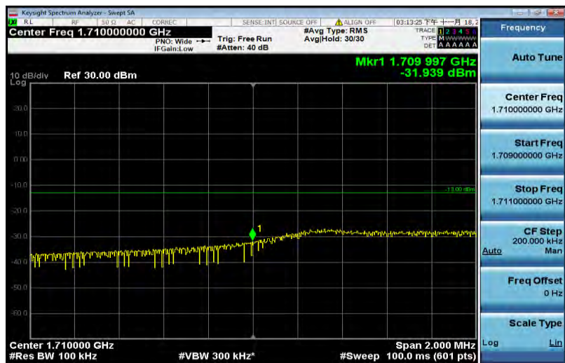
Band4-5MHz-QPSK-19975-25RB#0
