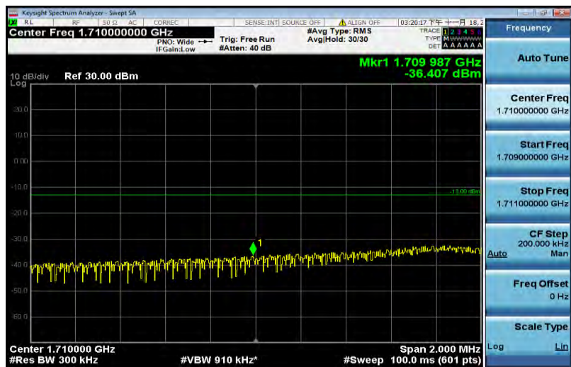
Band4-15MHz-16QAM-20025-75RB#0
