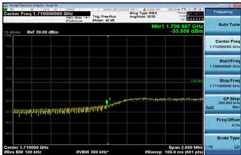
Band4-5MHz-16QAM-19975-25RB#0
