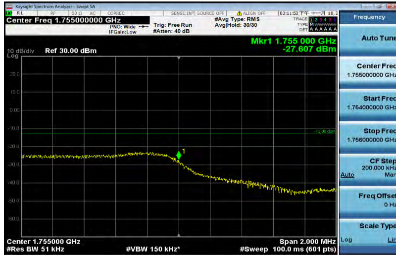
Band4-3MHz-QPSK-20385-1RB#14
