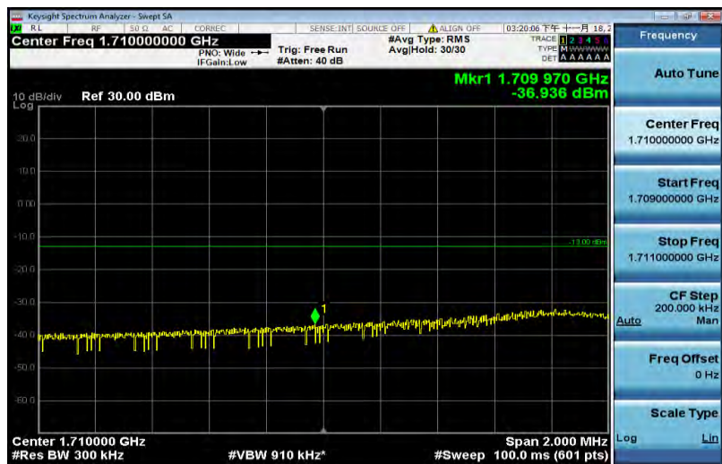
Band4-15MHz-QPSK-20025-75RB#0
