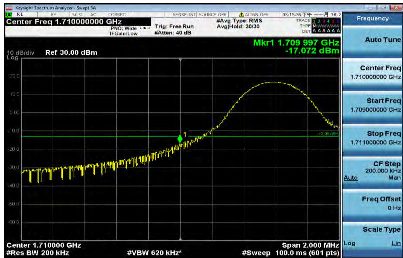
Band4-10MHz-QPSK-20000-1RB#49
