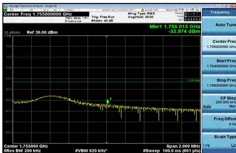
Band4-10MHz-16QAM-20350-50RB#0
