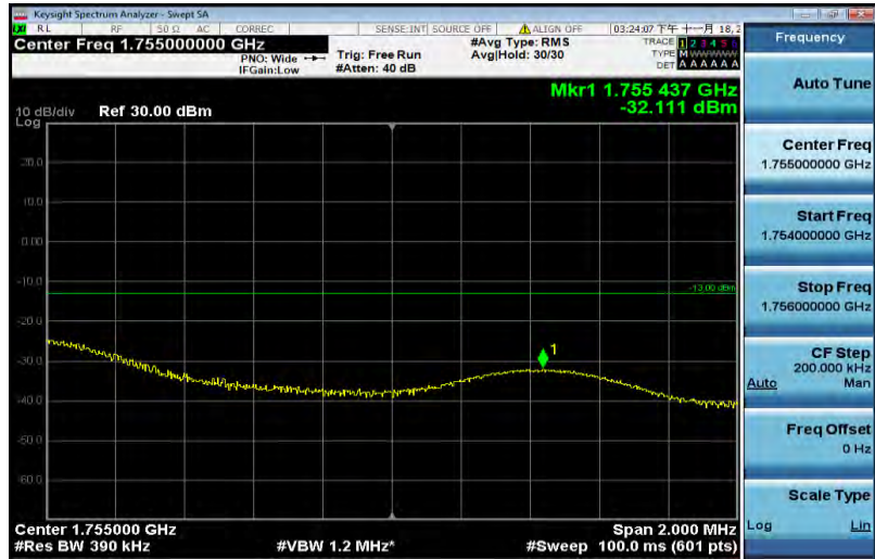
Band4-20MHz-16QAM-20300-1RB#99
