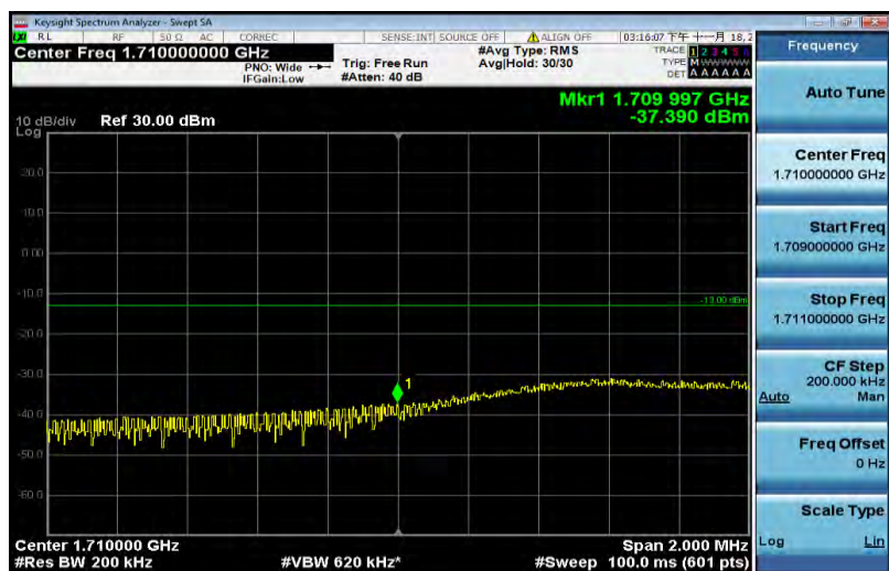
Band4-10MHz-16QAM-20000-50RB#0
