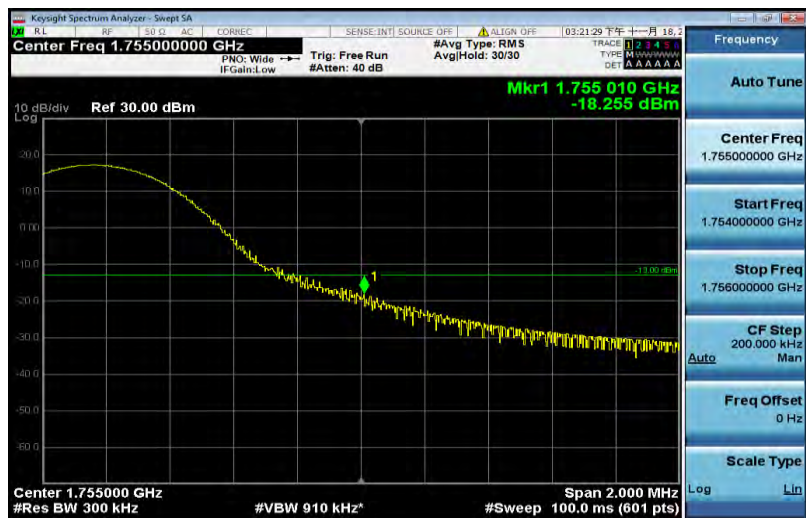
Band4-15MHz-QPSK-20325-75RB#0
