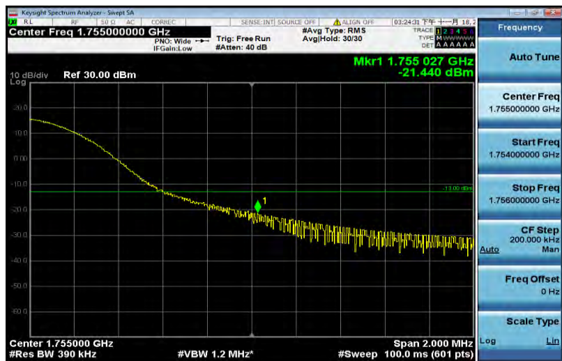
Band4-20MHz-16QAM-20300-100RB#0
