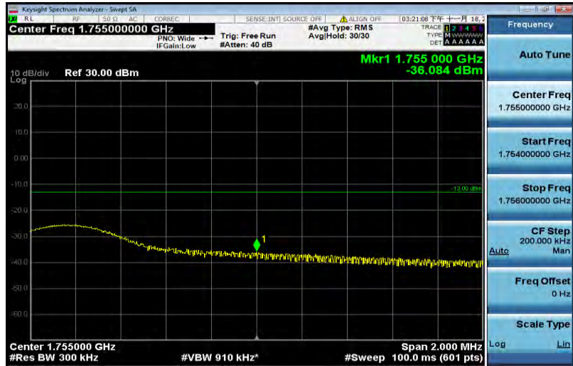
Band4-15MHz-QPSK-20325-1RB#74
