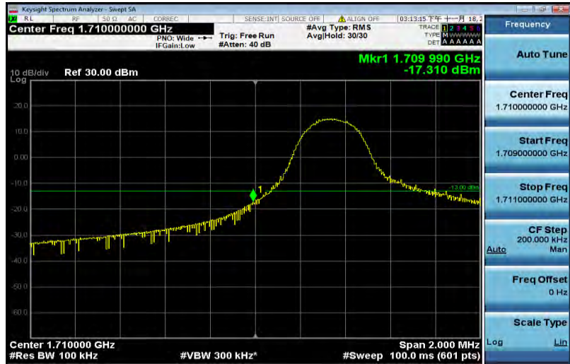
Band4-5MHz-16QAM-19975-1RB#24
