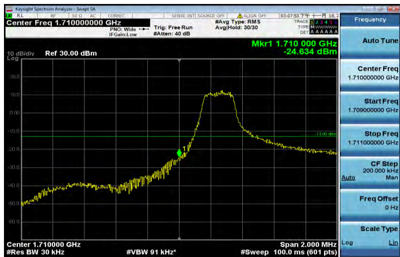
Band4-1.4MHz-16QAM-19957-6RB#0
