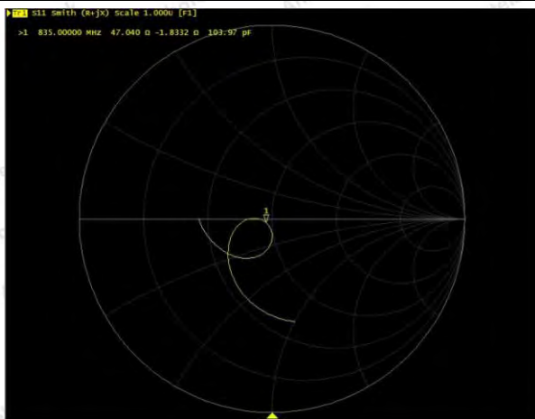
Impedance Test-Body
