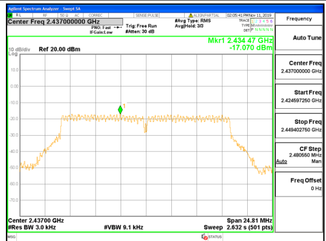
Channel 6 / 2437 MHz
