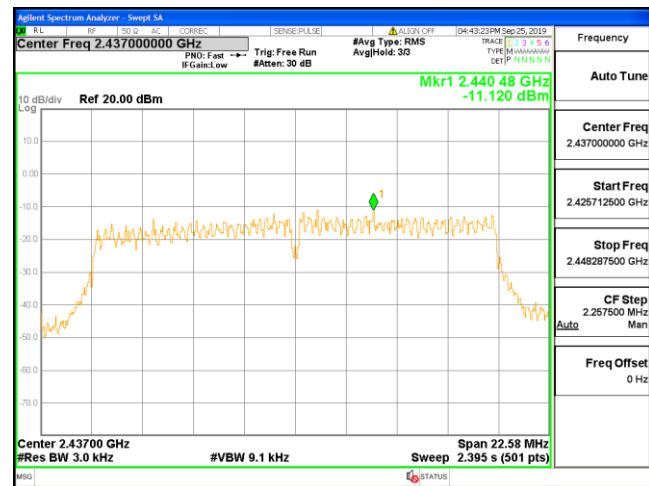
Channel 6 / 2437 MHz
