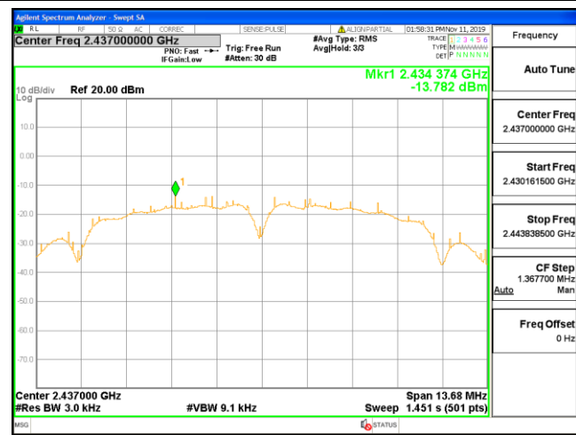
Channel 6 / 2437 MHz
