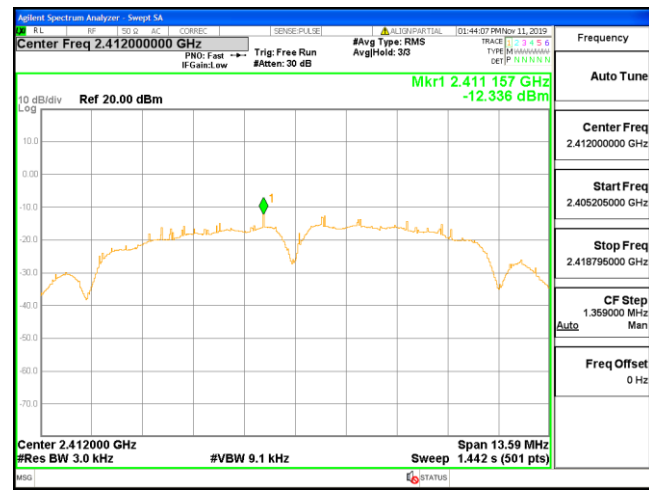
Channel 1 / 2412 MHz
