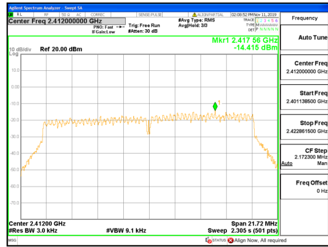
Channel 1 / 2412 MHz
