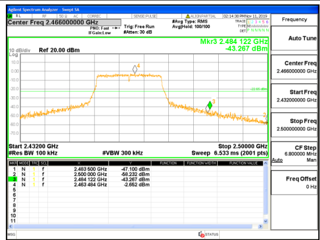
Channel 11 / 2462 MHz
