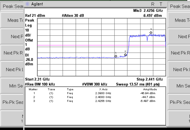
Low bandedge Plot
