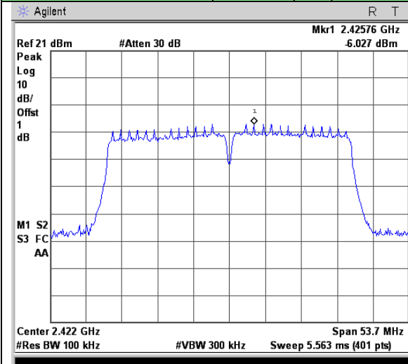
100KHz PSD Reference Level
