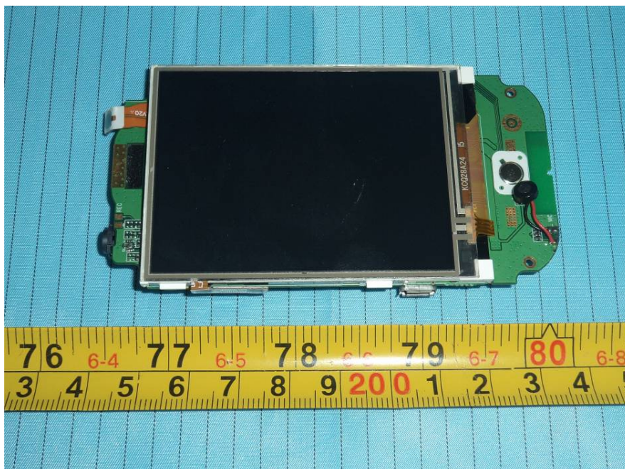
EUT – Main Board with Display Top View
