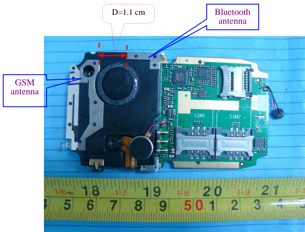
Antenna Location
