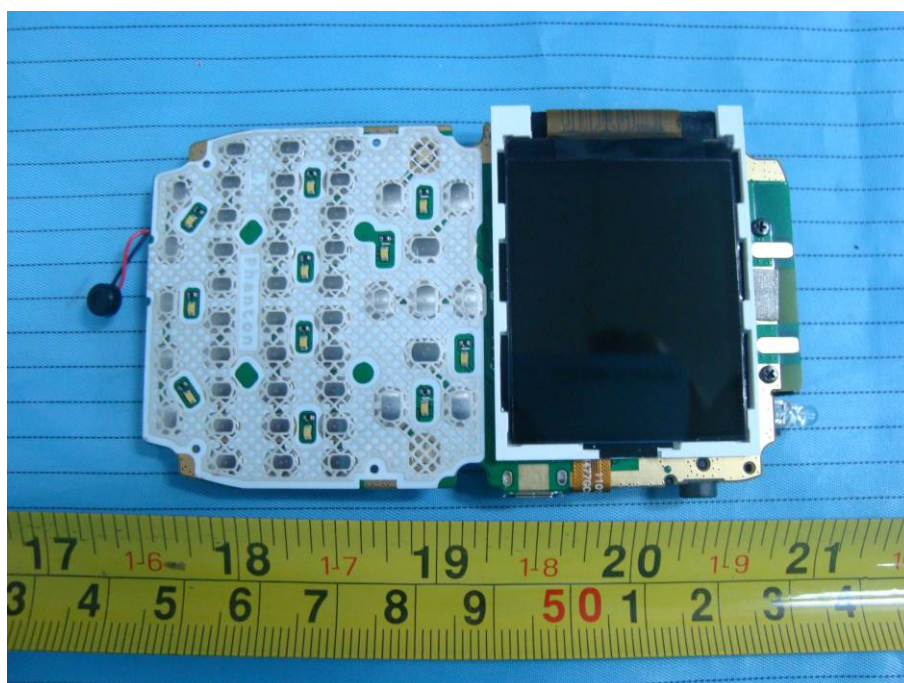
EUT – Main Board Bottom View with LCD
