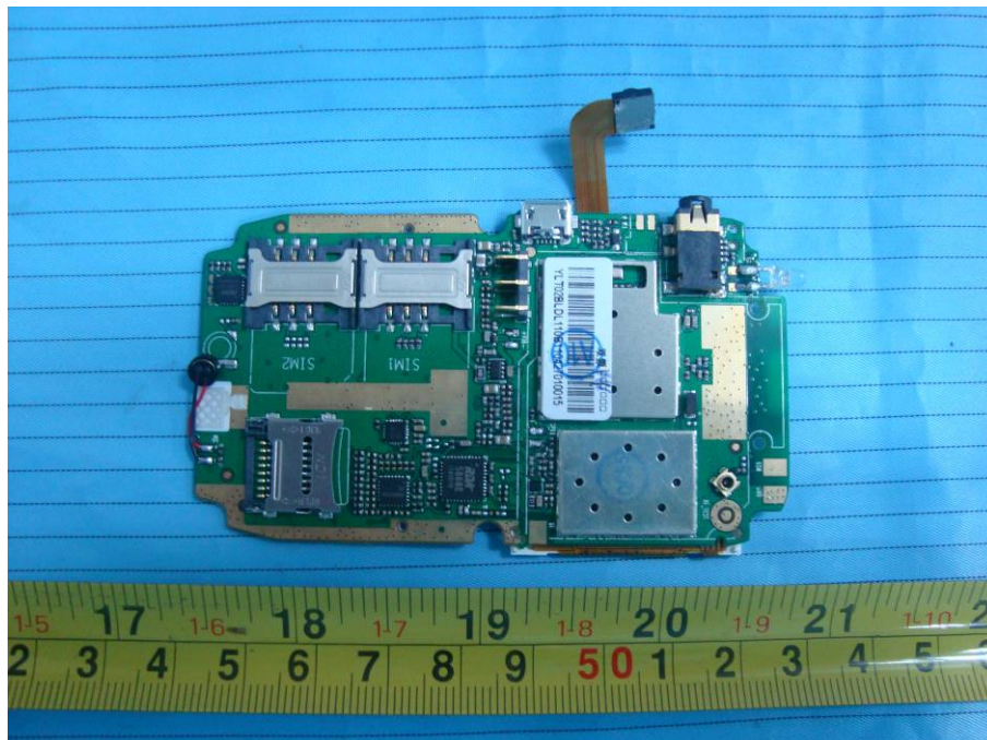
EUT – Main Board Top View without Antenna
