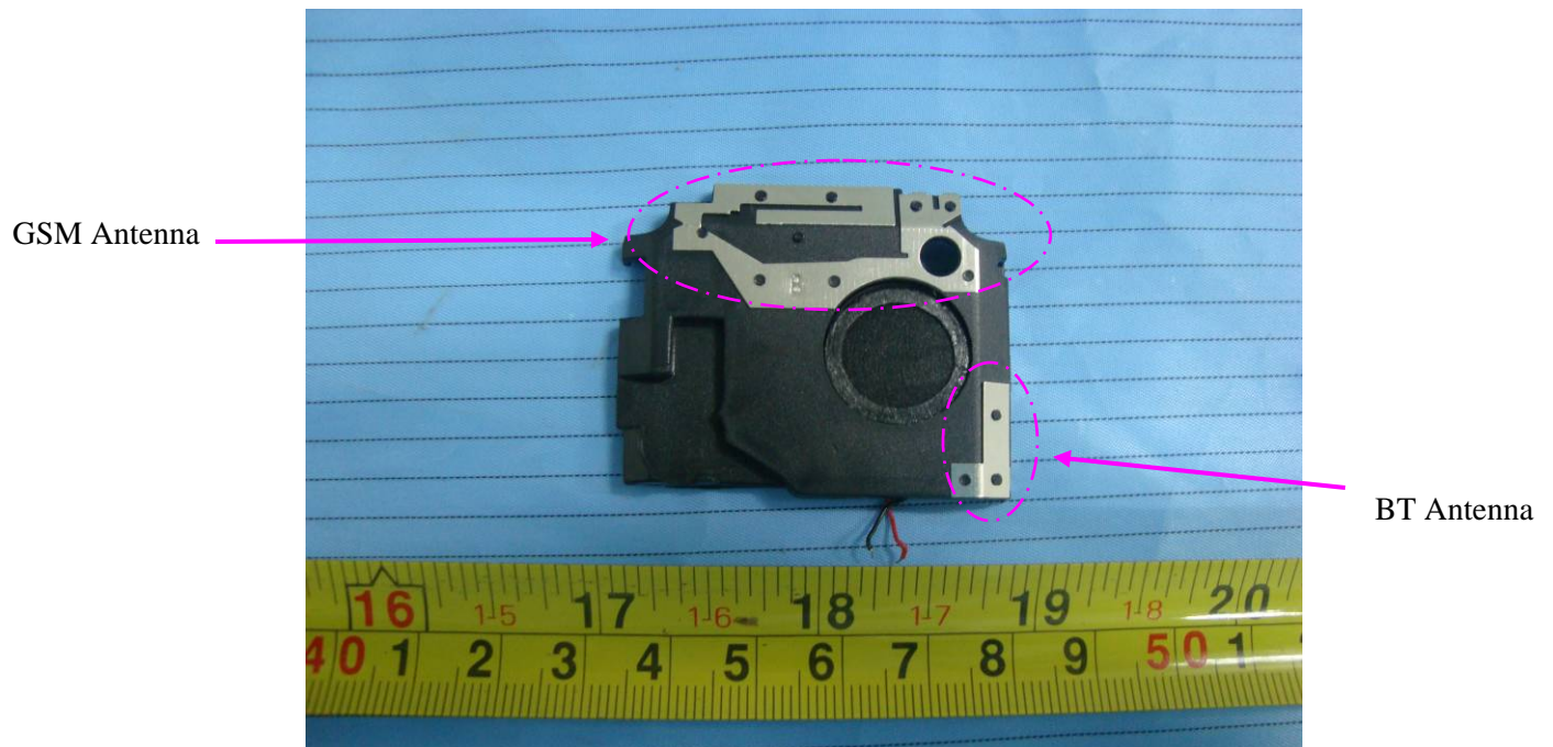
EUT – Antenna View
