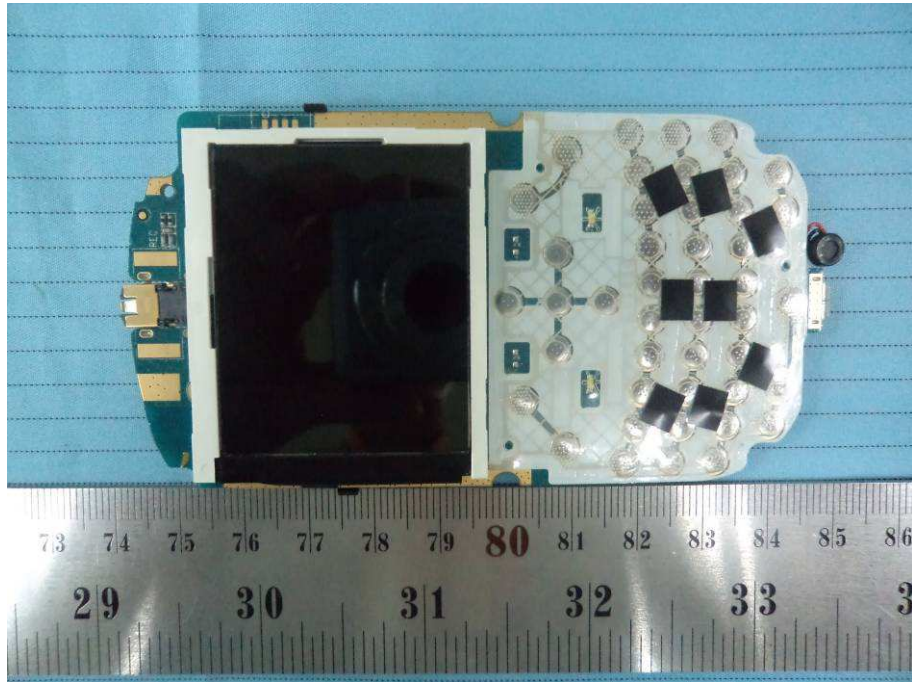
EUT – Main Board Top with LCD and Keyboard Top View
