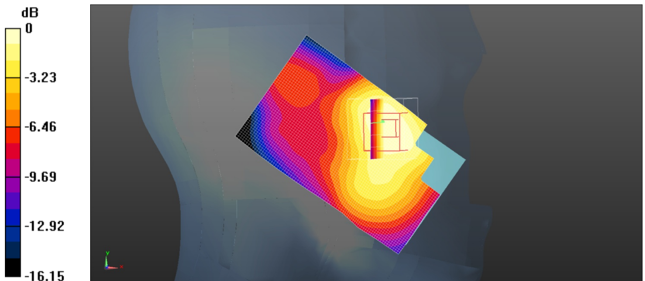
Left Head Tilt (PCS1900 Middle Channel)
