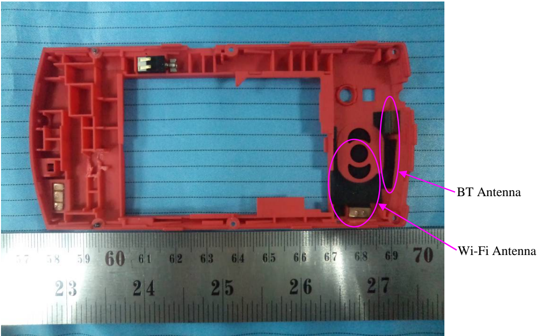
EUT – BT & Wi-Fi Antenna View
