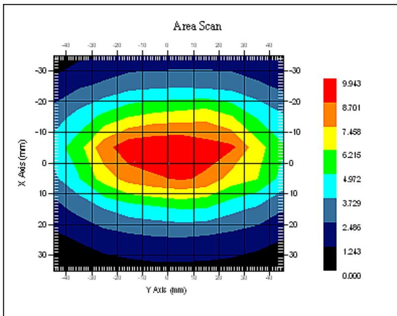
835 MHz System Validation with Head Tissue
