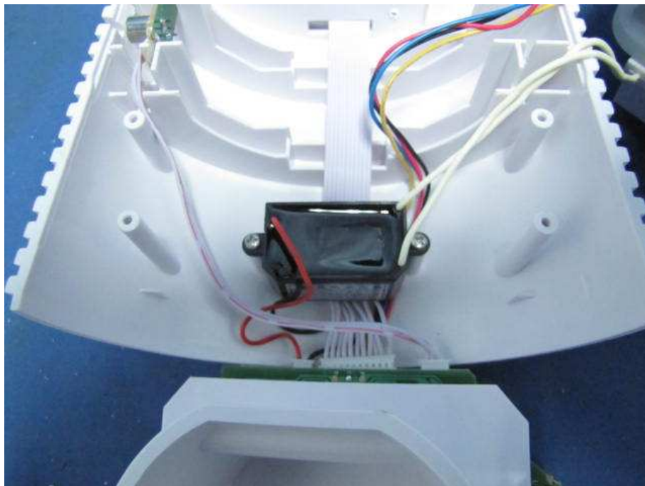
Inside view4 for Air Purifier
