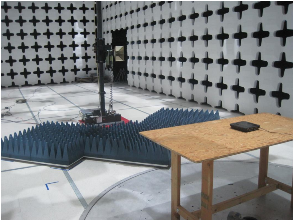
Radiated Emission Above 1 GHz Back View
