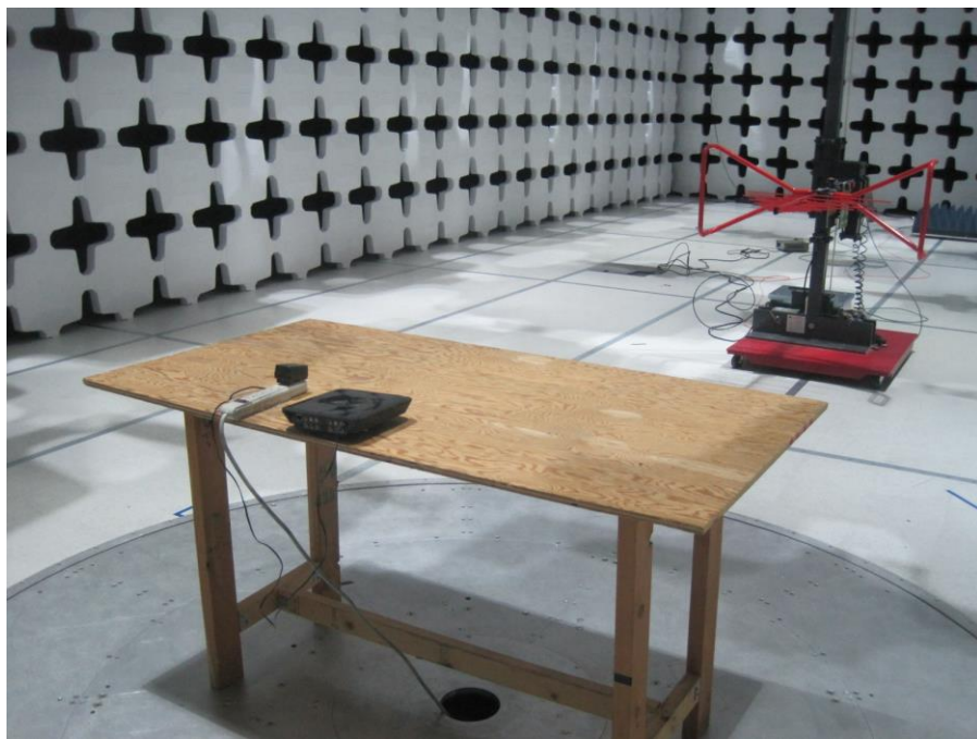
Part 15C Radiated Emission Below 1 GHz Back View
