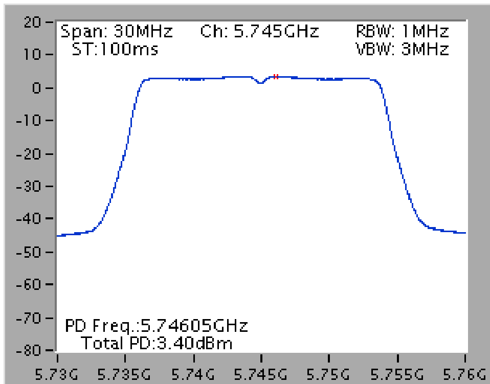
Power Density Plot on Configuration IEEE 802.11ac MCS0/Nss1 VHT20 / Ant. 1 + Ant. 2 + Ant. 3 / 5745 MHz
