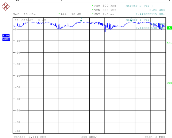
Fig.80 Carrier separation measurement: \pi/4 DQPSK, Ch39
