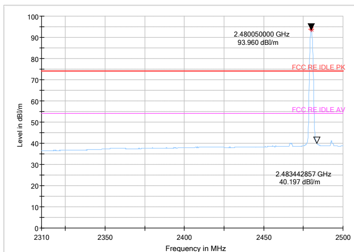
BANDEDGE: 8DPSK, Ch78,AVG
