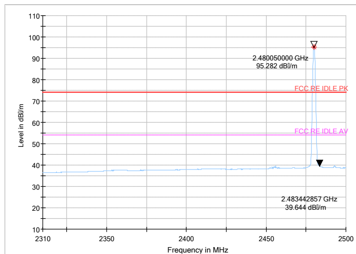
BANDEDGE: GFSK, Ch78,AVG
