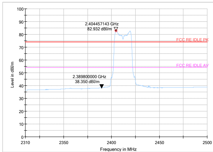
Fig.73 Radiated emission (Power): 802.11n, low channel
