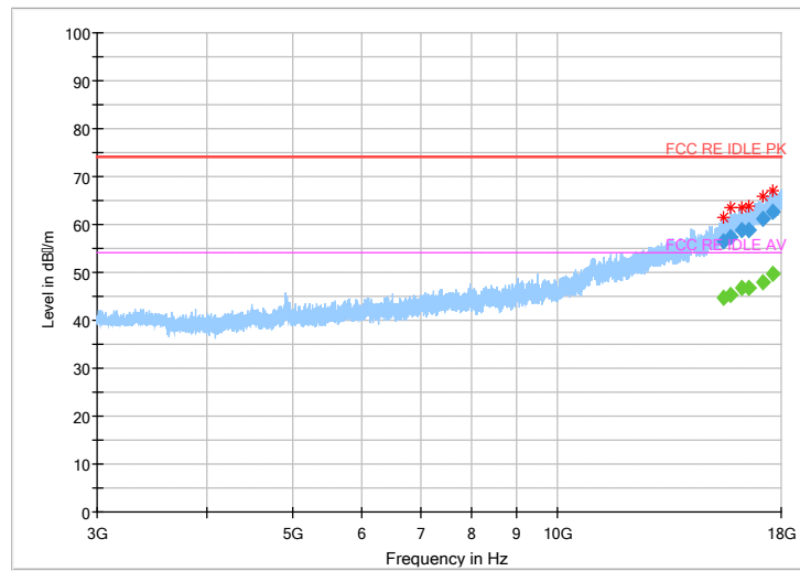
Fig.61 Radiated Spurious Emission (802.11g,Ch11,3GHz~18GHz)
