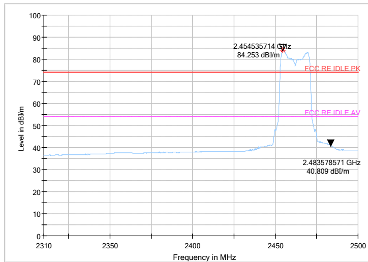
Fig.74 Radiated emission (Power): 802.11n, channel 11
