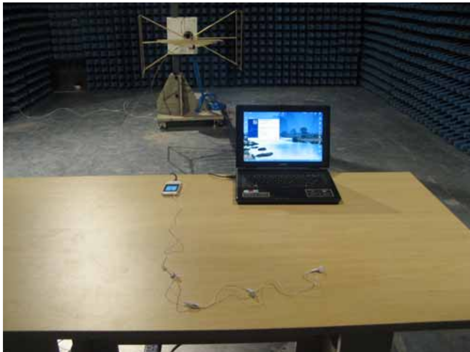
FCC RADIATED EMISSION TEST SETUP FOR PC MODE
