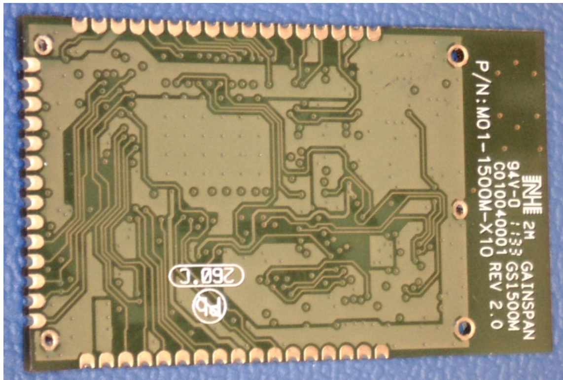
Figure 2 Internal Bottom View
