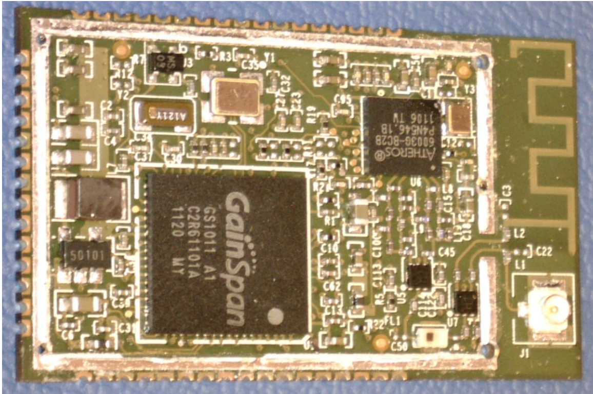
Figure 1 Internal Top View
