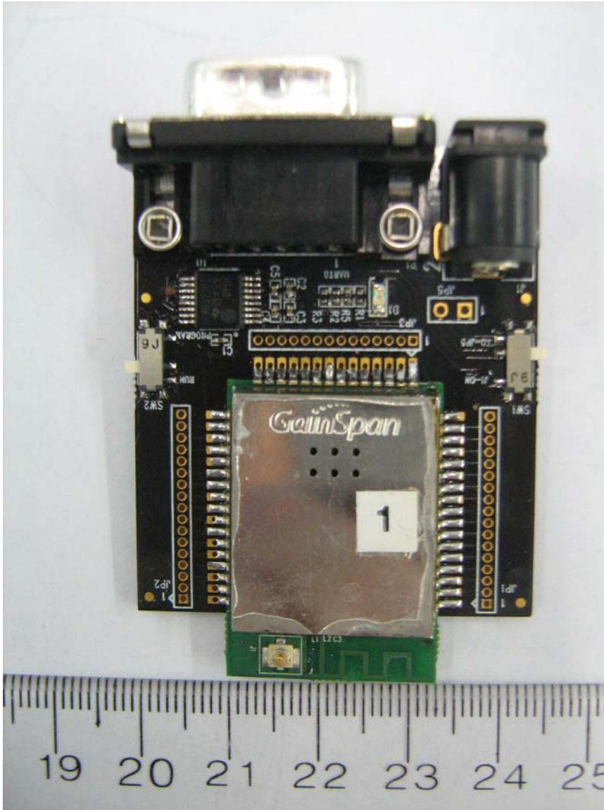
Figure 1: External Photo of GS1011MIP WiFi Module on the Support Card (Component Side)
