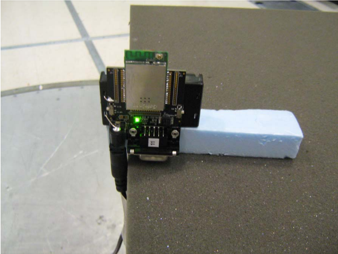
Figure 9: Radiated Emission Setup on Z-Axis
