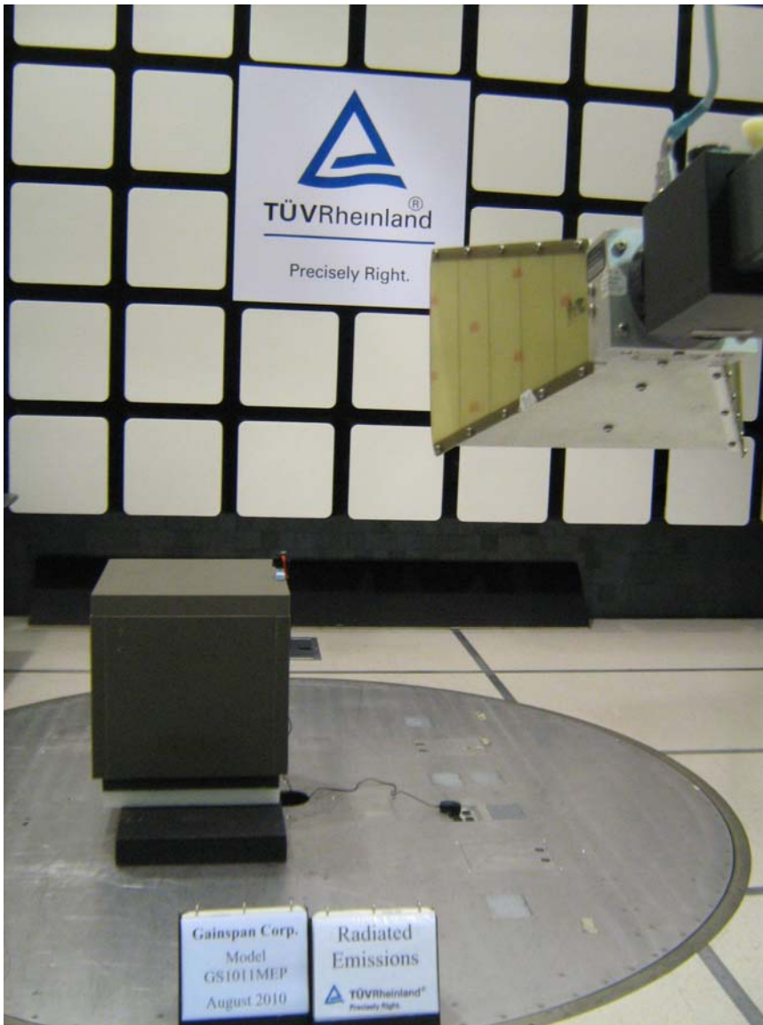
Figure 4: Radiated Emission Test Setup for 1GHz to 18GHz (Rear View)
