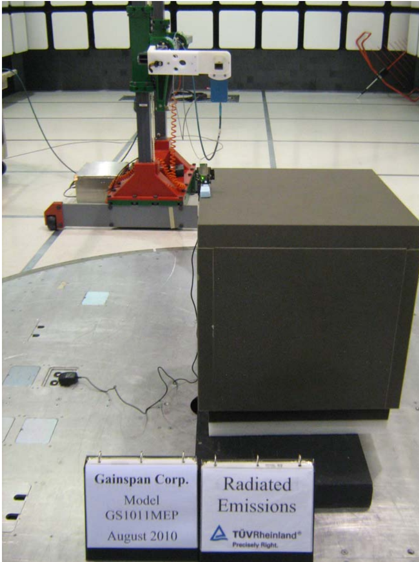
Figure 5: Radiated Emission Test Setup for 18 GHz to 26GHz (Front View)
