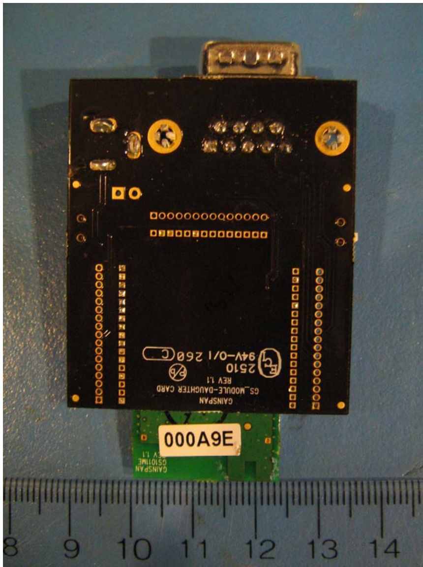
Figure 2: External Photo of GS1011MEP WiFi Module on the Support Card (Soldered Side)
