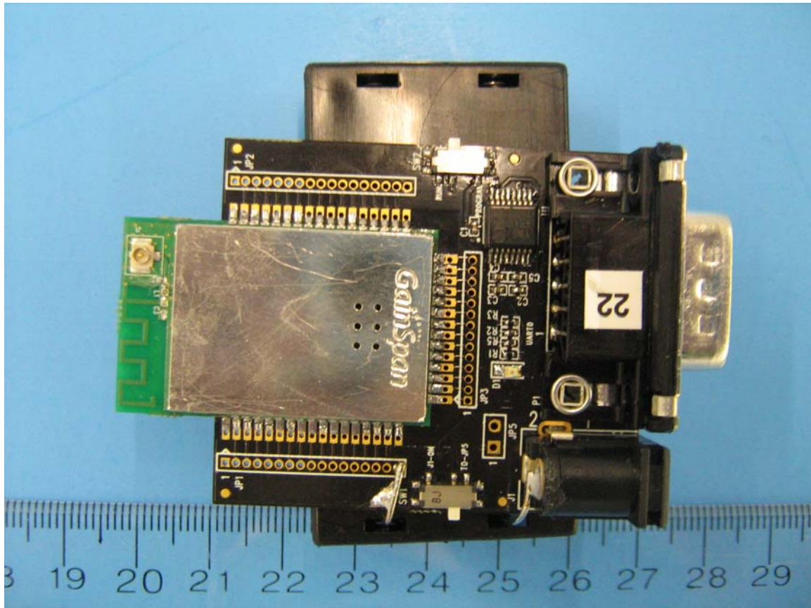
Figure 1: External Photo of GS1011MEE WiFi Module on the Support Card (Component Side)
