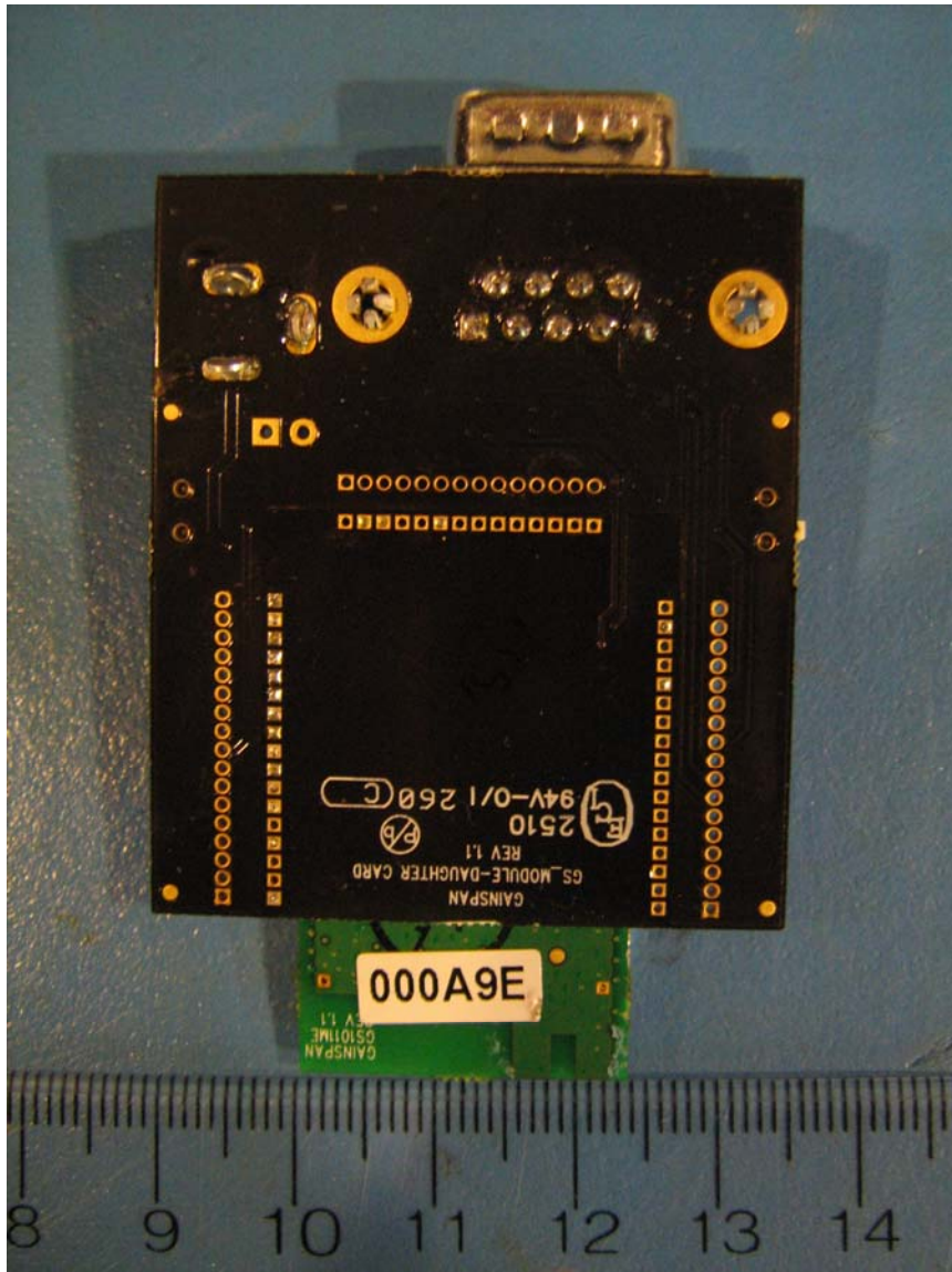
Figure 2: External Photo of GS1011MEE WiFi Module on the Support Card (Soldered Side)
