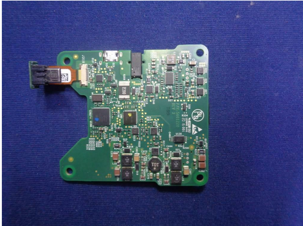
1 st PCB Top view
