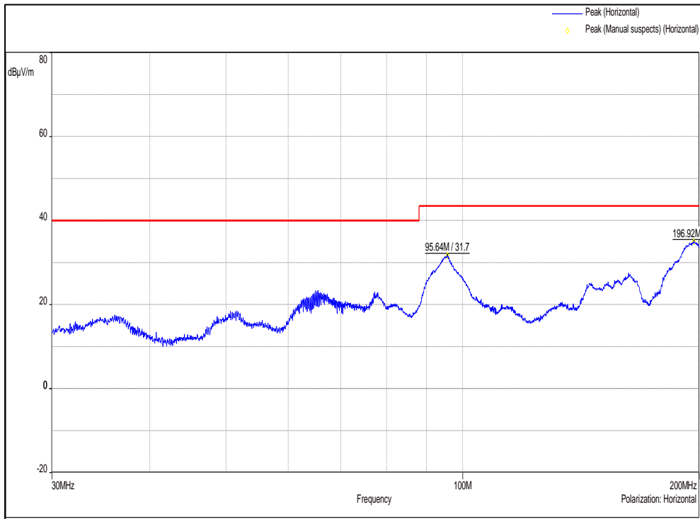
Channel Frequency 30MHz – 200MHz
