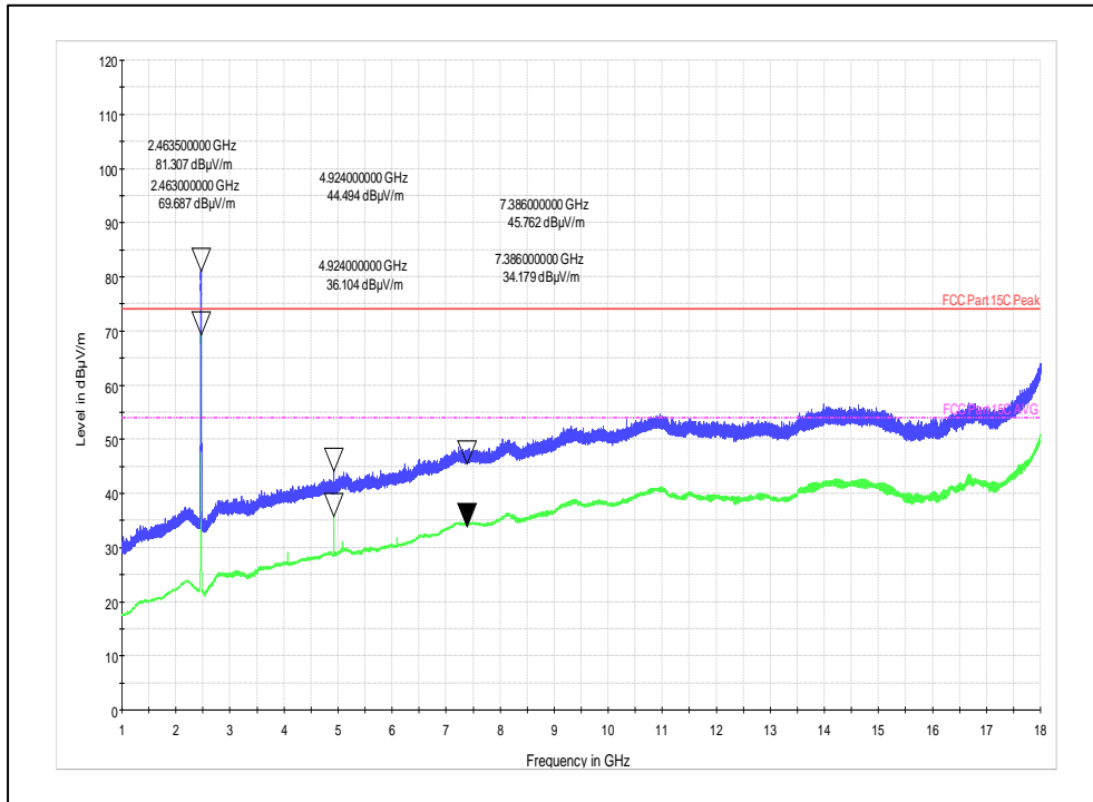
Channel Frequency: 1 – 18 GHz
