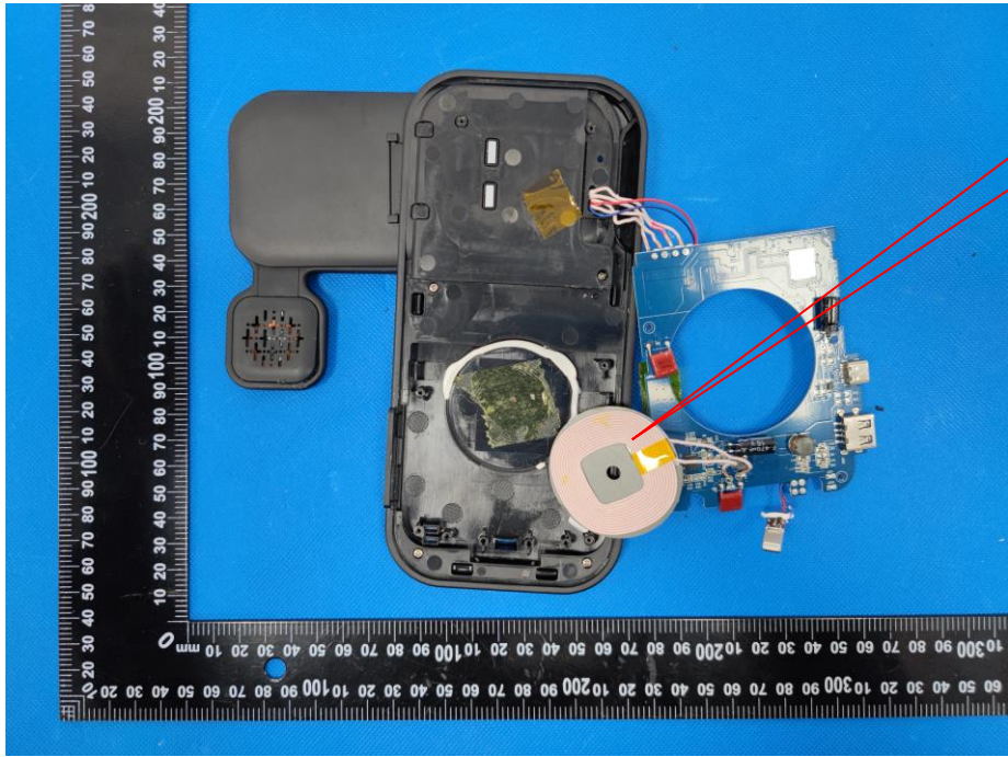
Phone 2 Antenna
