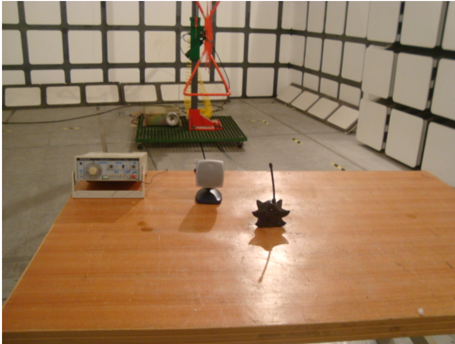
Radiated Emissions - Stand View (Front)
