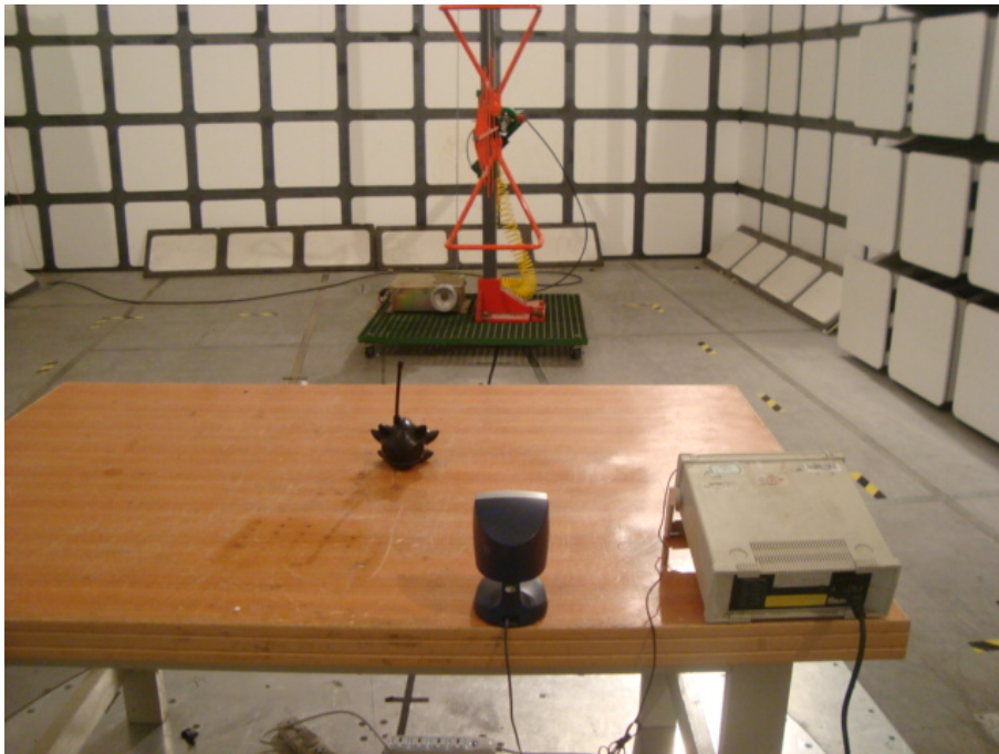
Radiated Emissions - Stand View (Rear)
