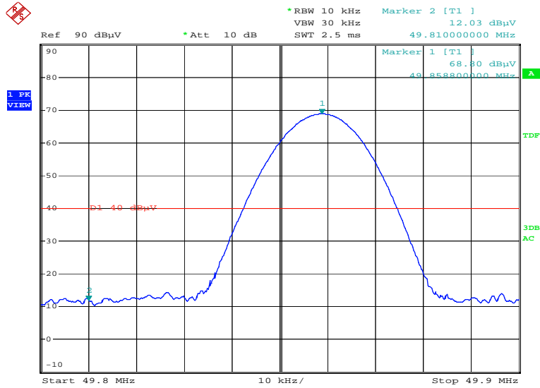
plot of band edge-left side Date: 16.AUG.2010 10:45:55
