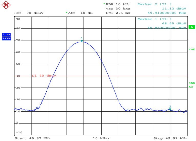
plot of band edge-right side Date: 16.AUG.2010 10:44:40
