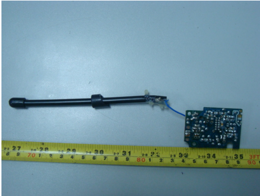
EUT – Mainboard with Antenna View 2
