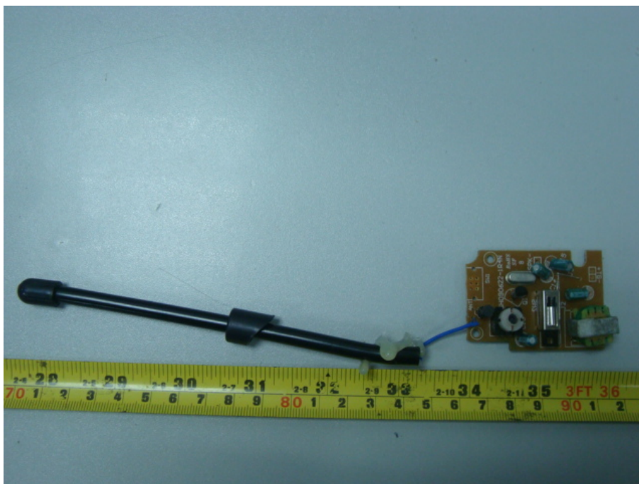
EUT – Mainboard with Antenna View 1
