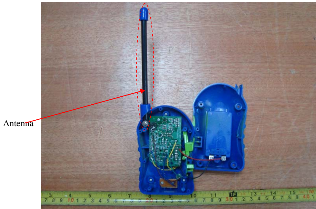
EUT – Battery off View
