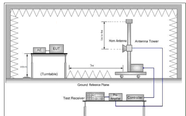
Figure 2. Above 1 GHz
