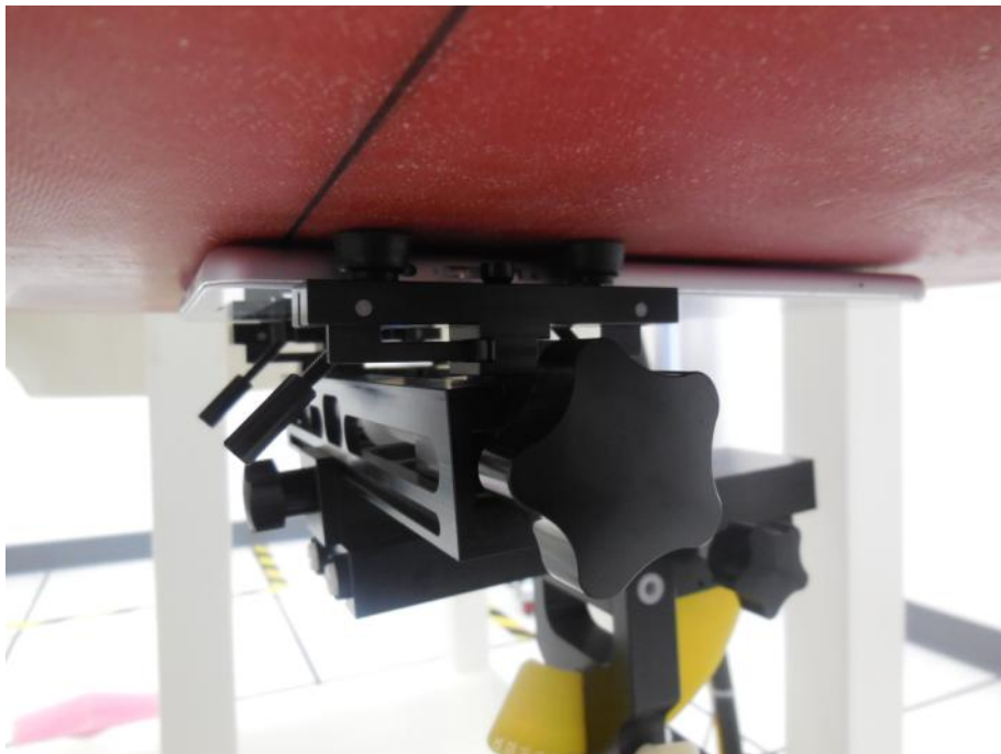
WIFI Test Setup Body Back with gap 0mm
