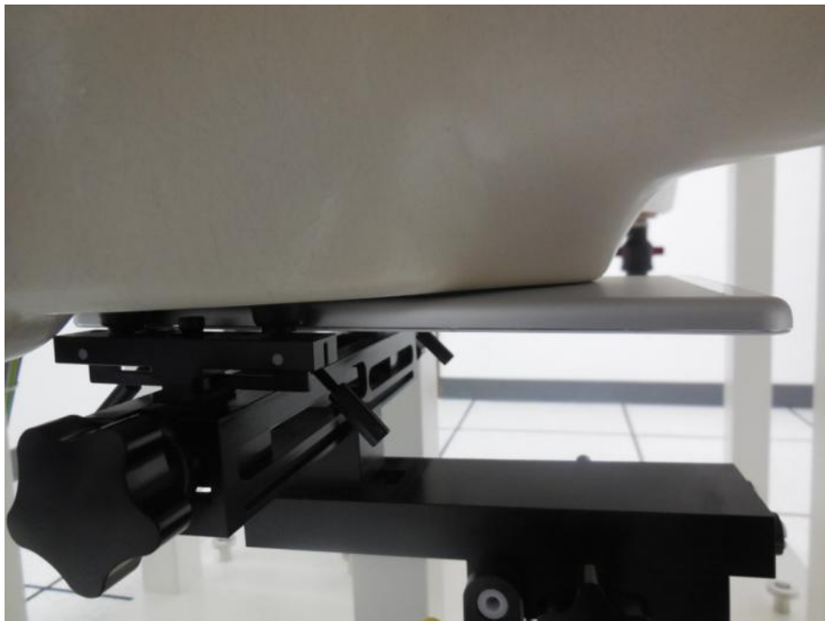
Band850 Test Setup Body Back with gap 0mm
