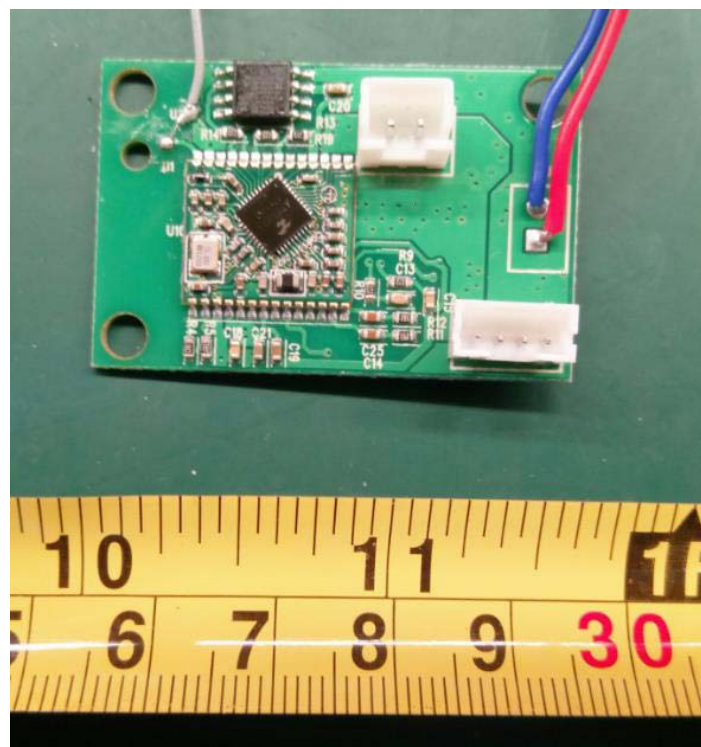
EUT –Main Board Top View
