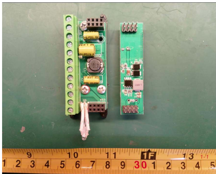
EUT – Power Board Top View
