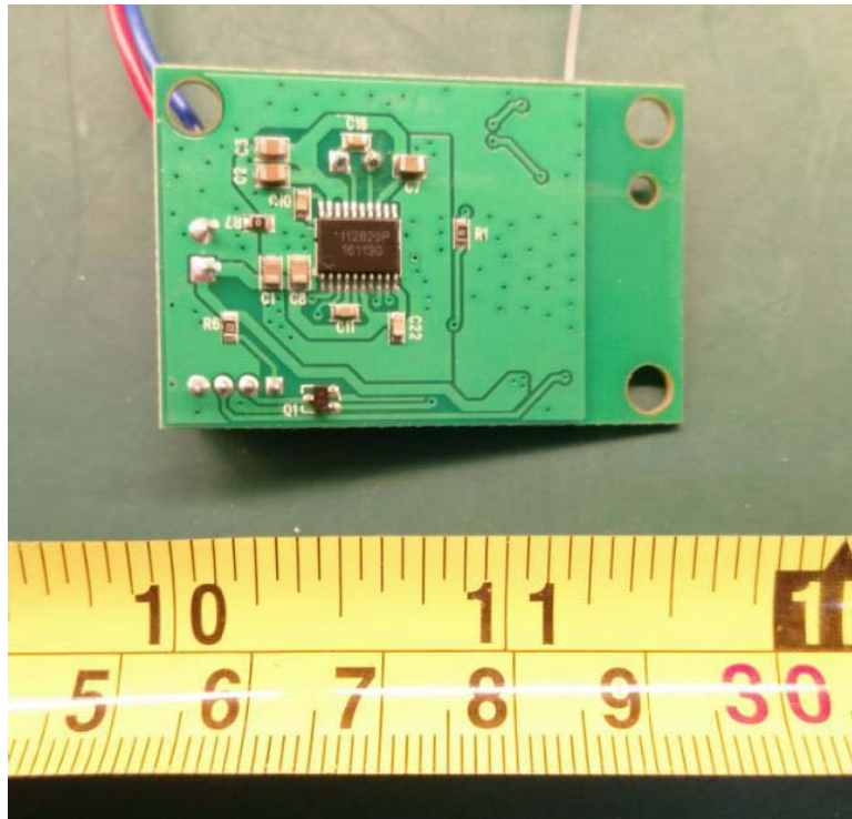
EUT –Main Board Bottom View
