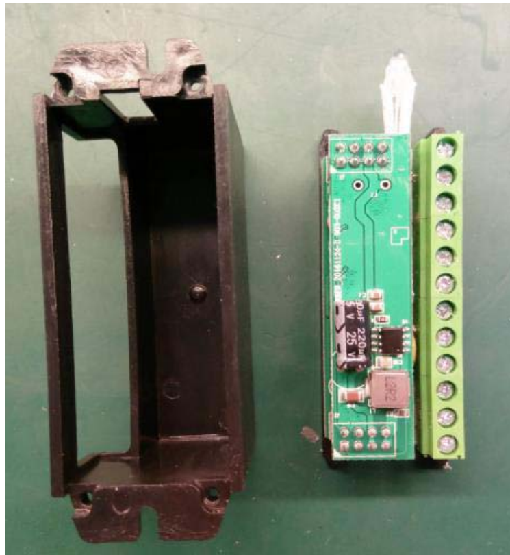
EUT – Power Uncover View
