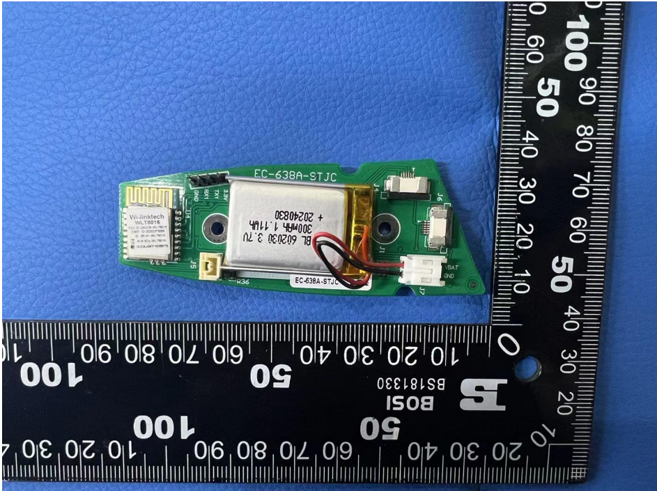
INTERNAL PHOTO OF SAMPLE PCB
