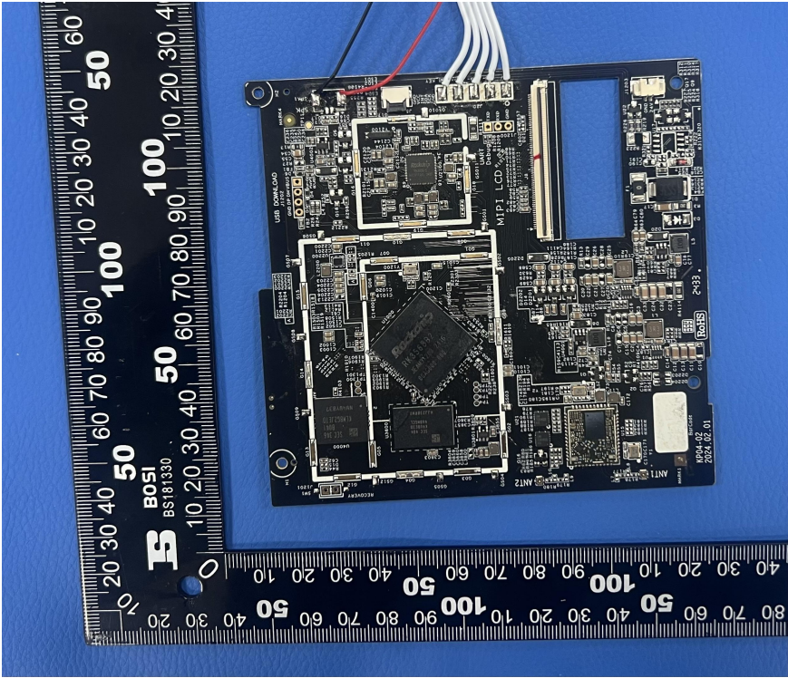
INTERNAL PHOTO OF SAMPLE PCB
