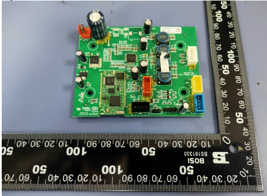
Solder Board-Component View 3
