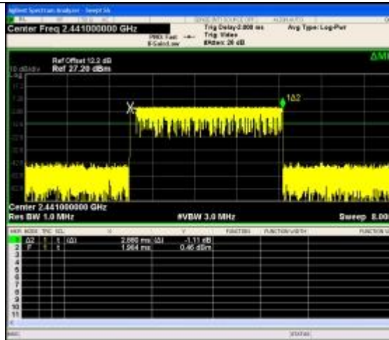
Pulse Width 8DPSK_3-DH5
