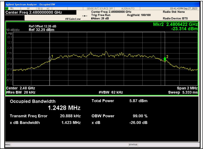
\pi/4 DQPSK_2-DH5_Channel 78
