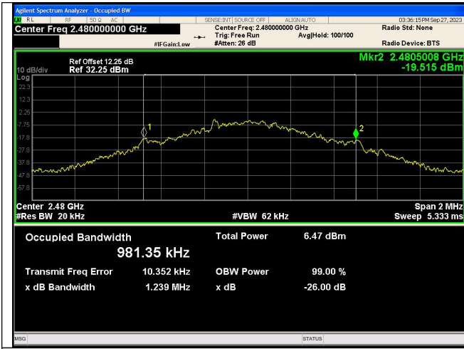
GFSK_DH5_Channel 78
