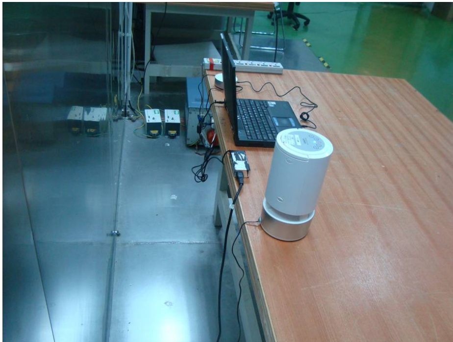
Conducted Emissions - Side View (with AC/DC adapter)
