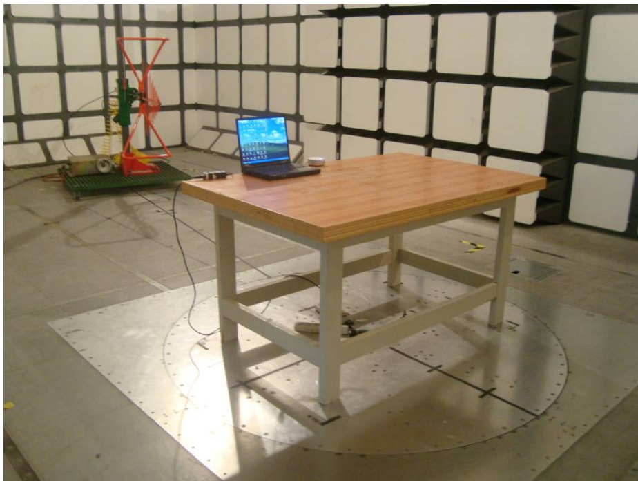
Below 1 GHz: Spurious Radiated Emissions - Rear View (via USB Port)
