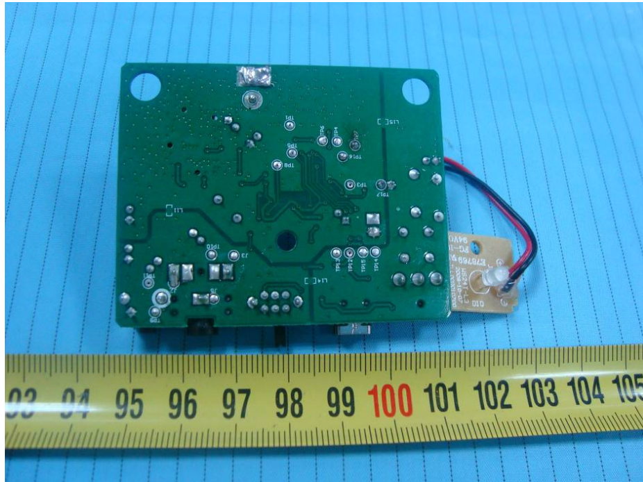
EUT – Main Board Bottom View (TX)
