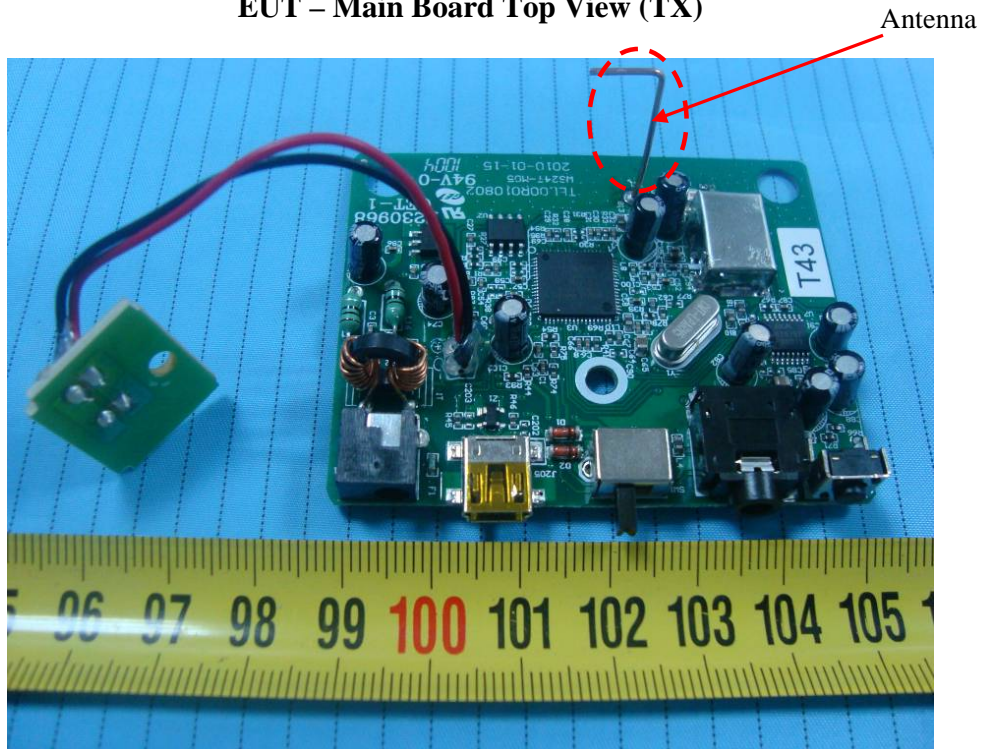
EUT – Main Board Top View (TX)
