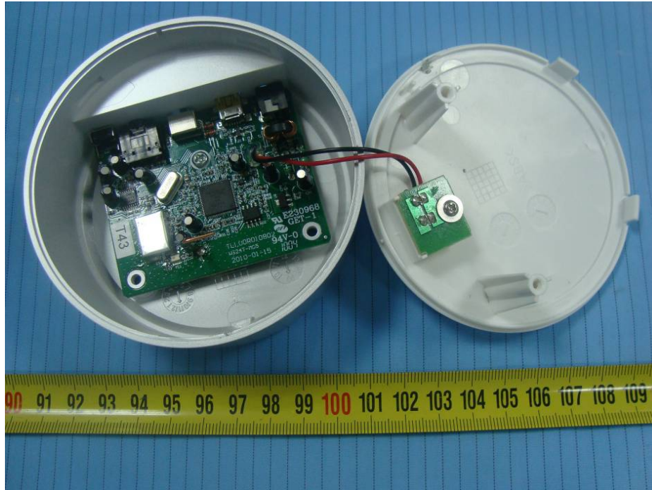
EUT – Main Board Top View (TX)
