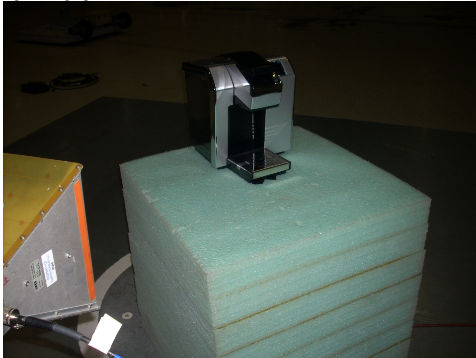
Radiated Emissions Measurements – Above 1GHz - OATS
