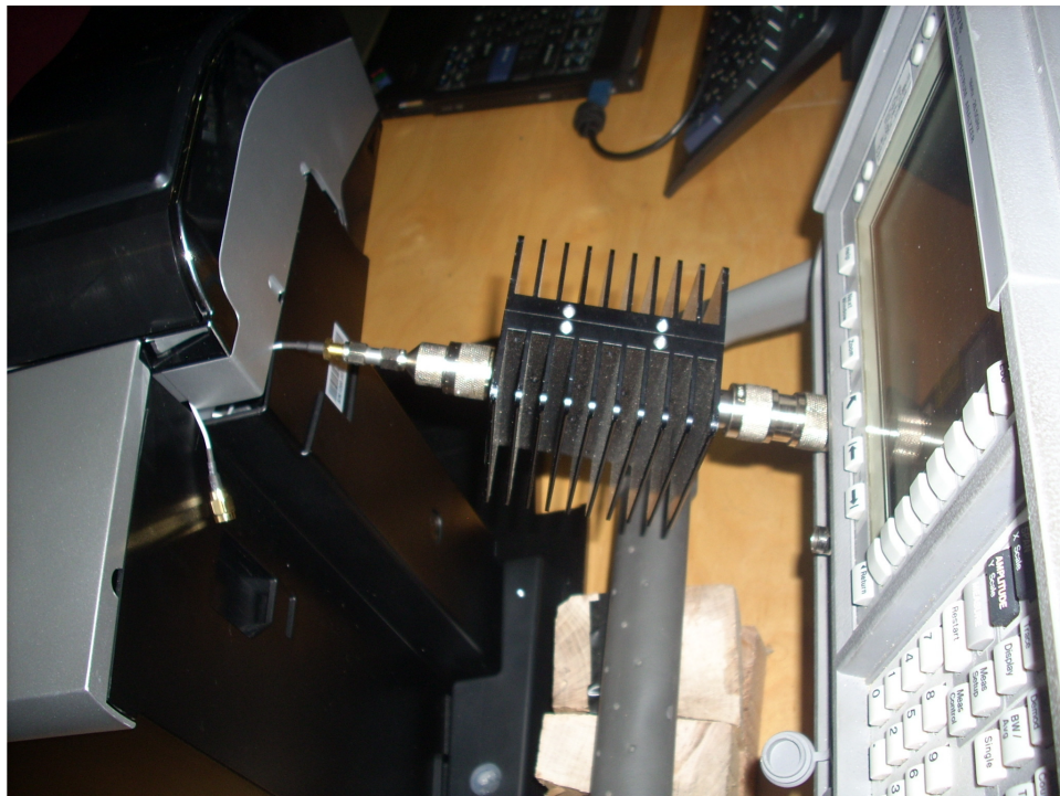
Conductive Measurements - Closeup
