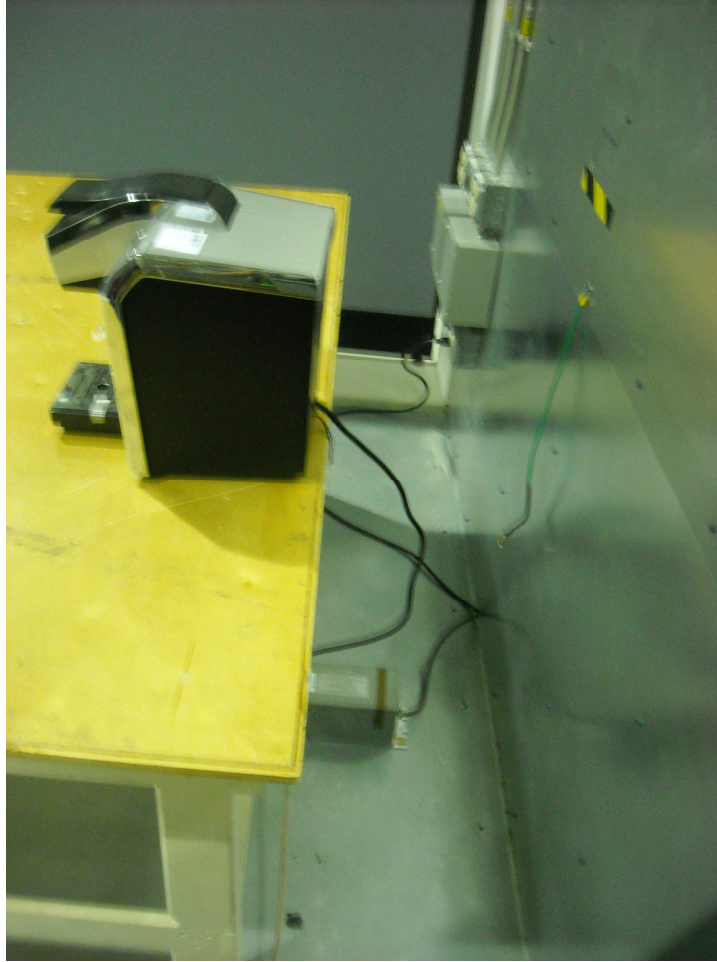
AC Line Conducted Emissions Measurements – Rear
