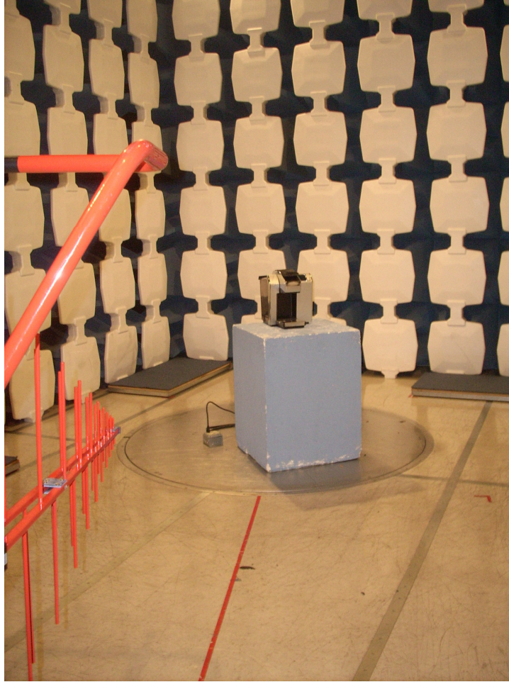
Radiated Emissions Measurements – Below 1GHz – Anechoic Chamber
