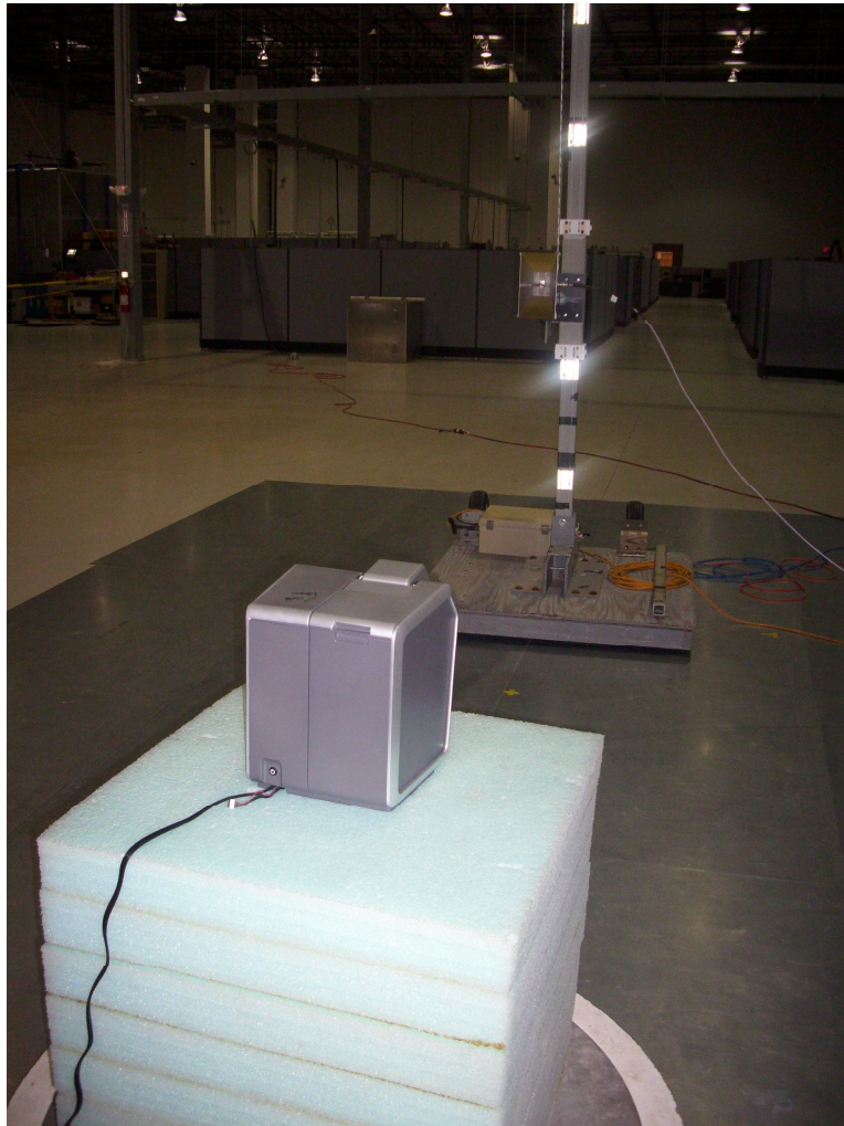
Radiated Spurious Emissions above 1GHz in OATS
