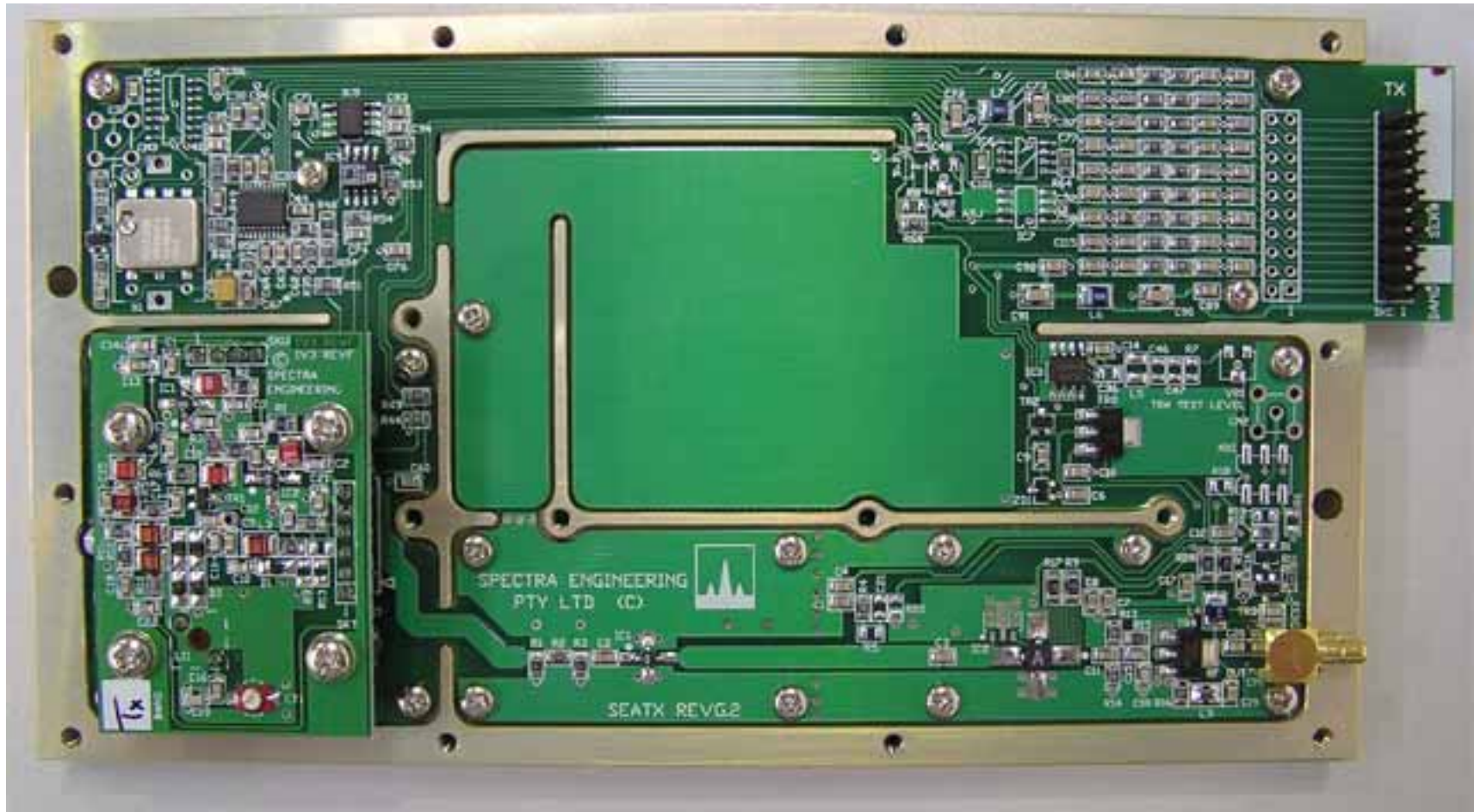
Top View Of Exciter
