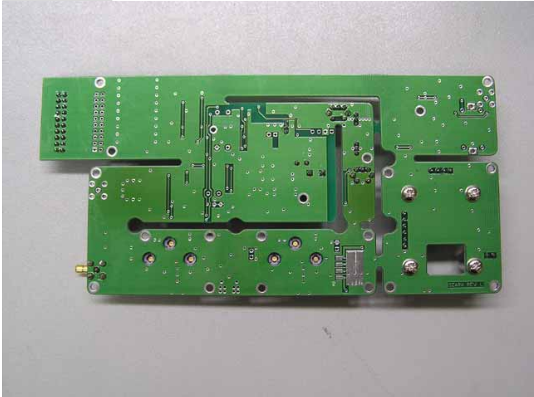
Bottom View Of Receiver PCB
