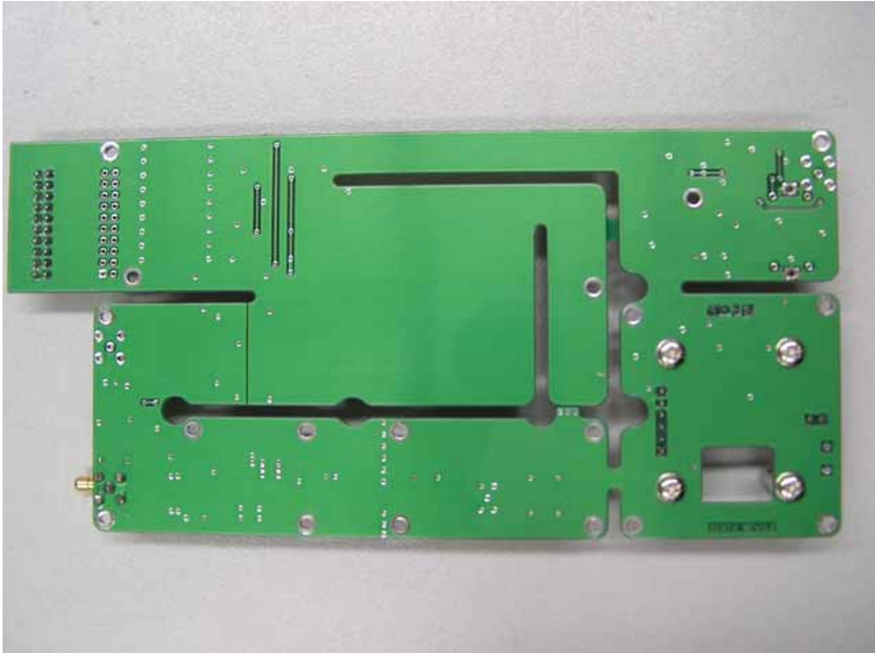
Bottom View Of Exciter PCB
