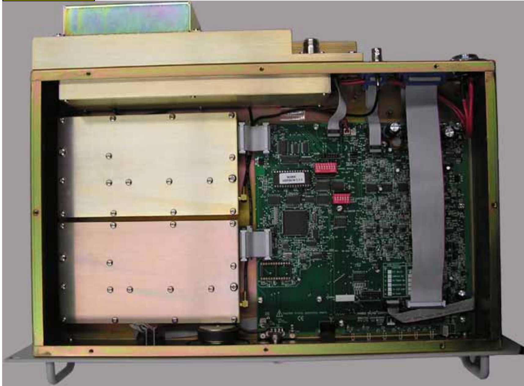
MX800 Complete Top View
