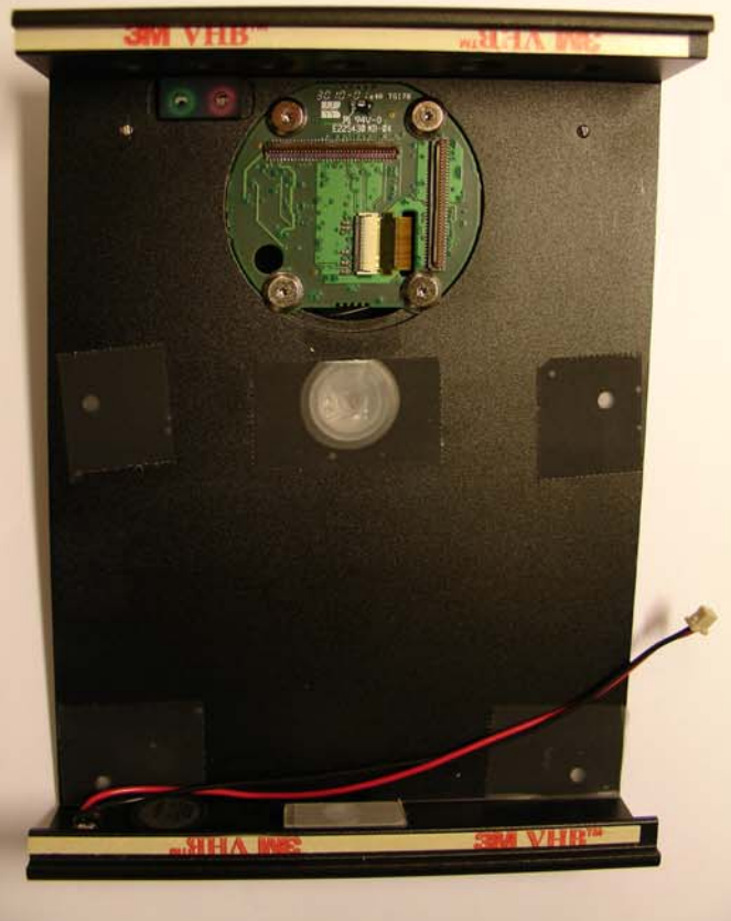
Camera board
