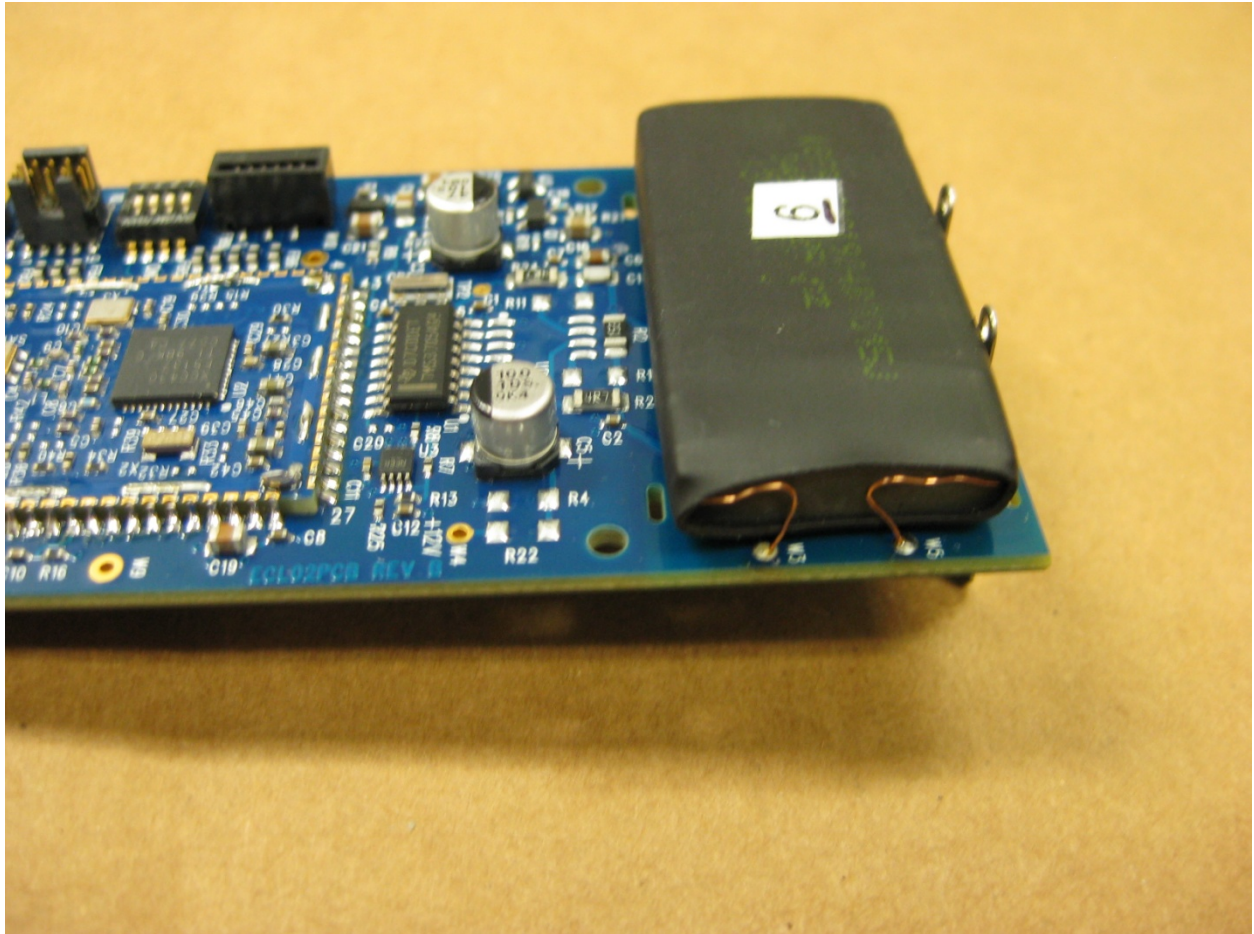
Close-up of Low Frequency RF Antenna
