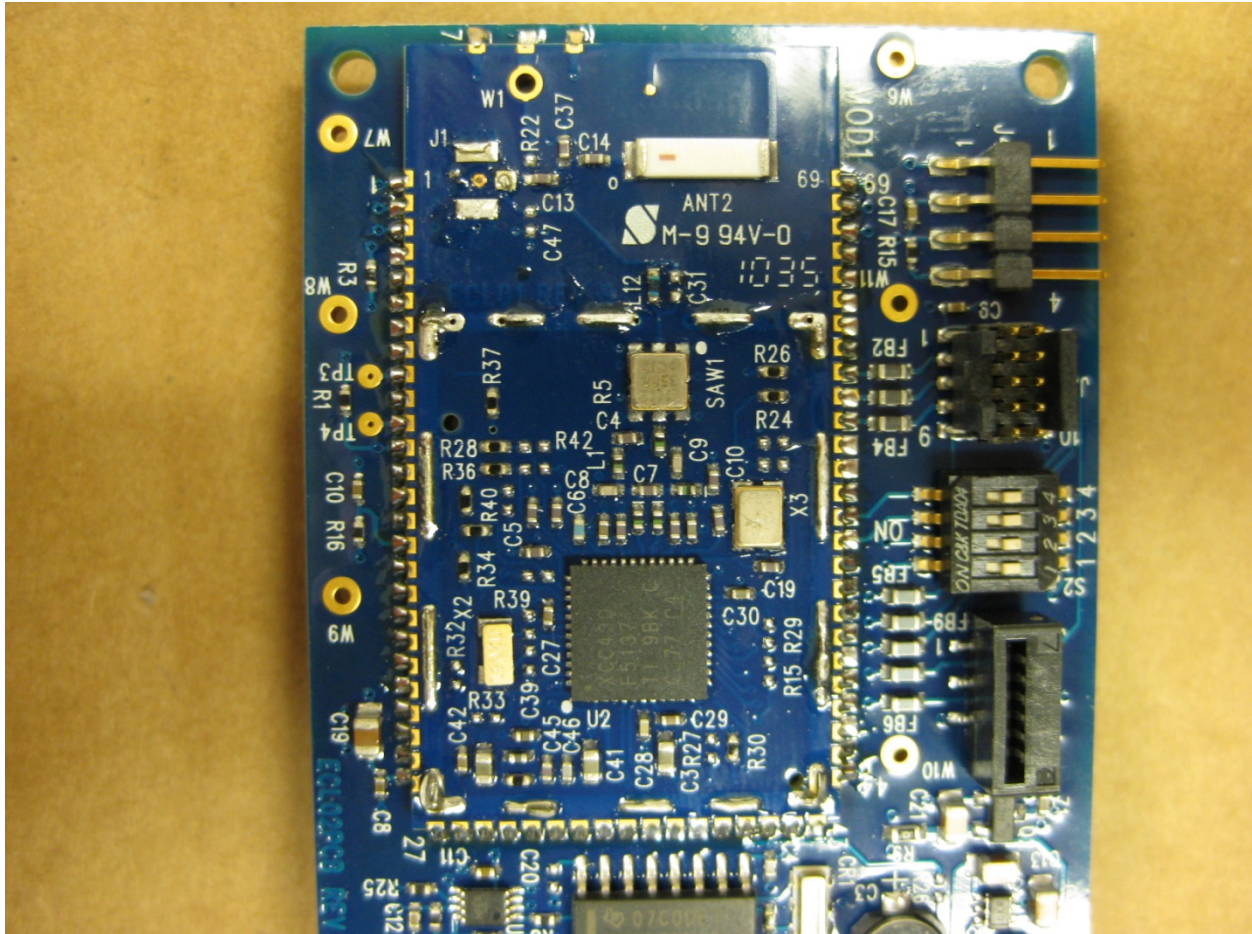
Close-up of RF Section with Shield Removed and Chip Antenna
